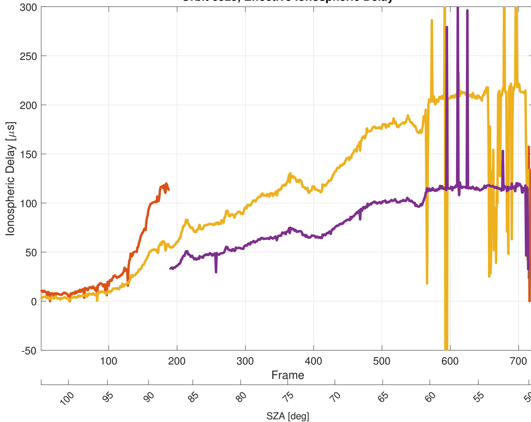
Orbit 6525, Effective Ionospheric Delay
