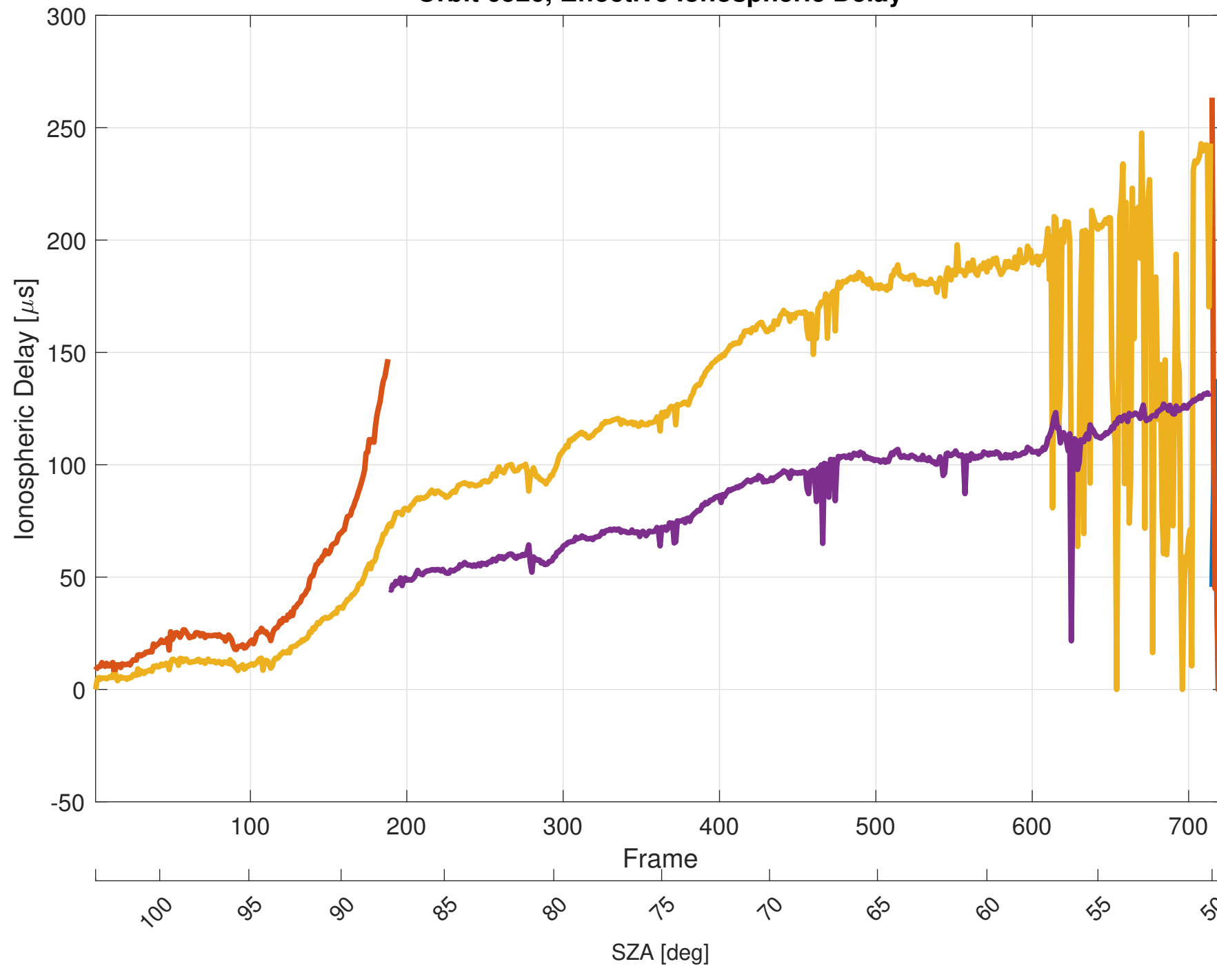
Orbit 6526, Effective Ionospheric Delay
