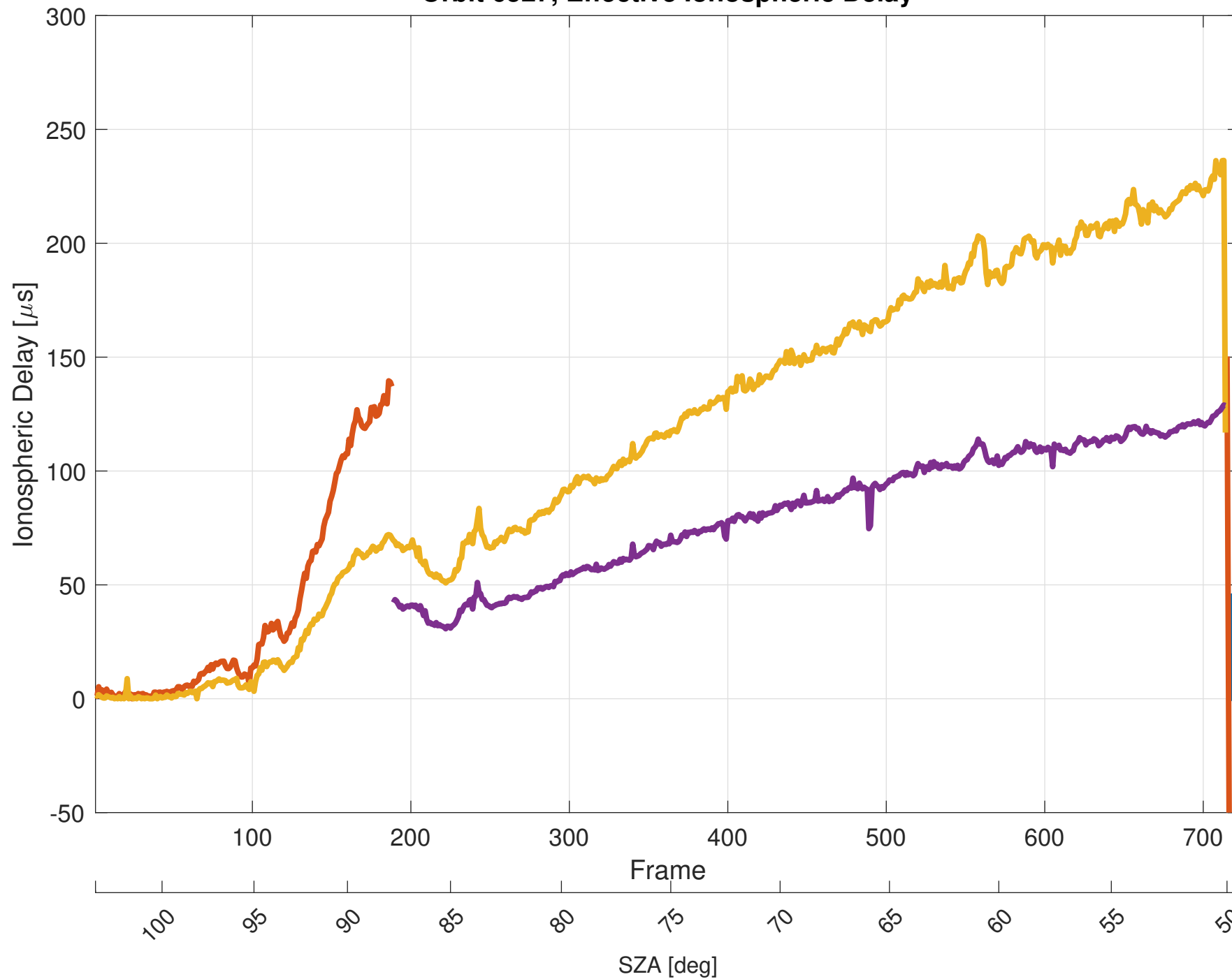
Orbit 6527, Effective Ionospheric Delay
