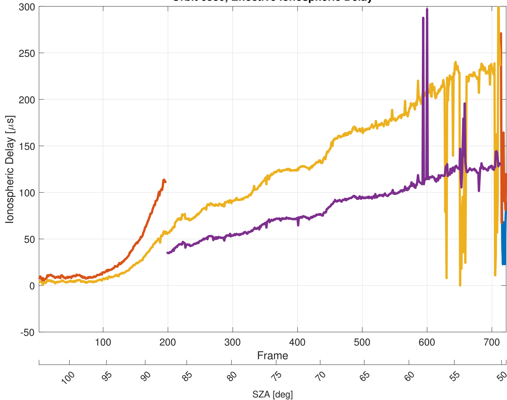
Orbit 6530, Effective Ionospheric Delay
