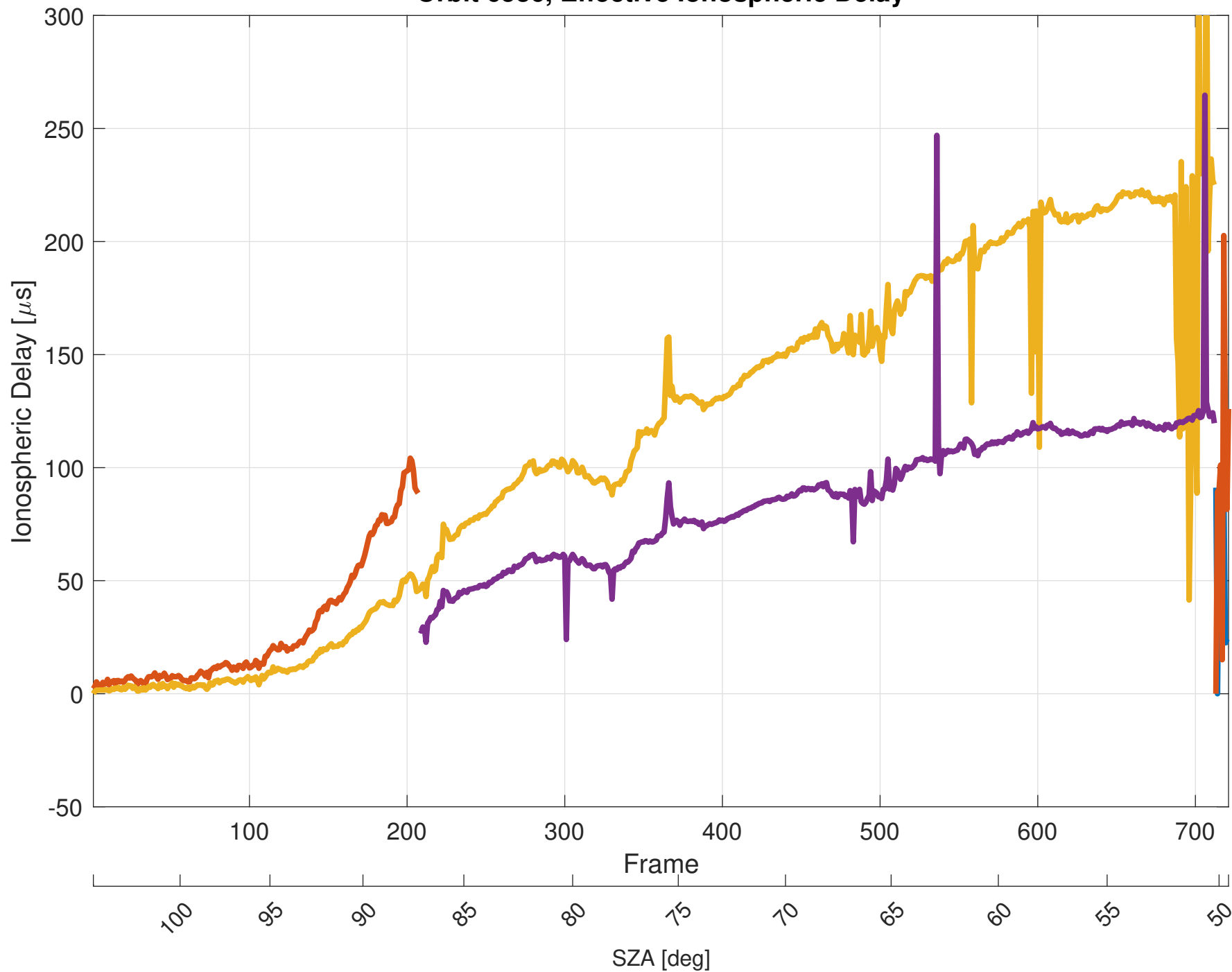
Orbit 6536, Effective Ionospheric Delay
