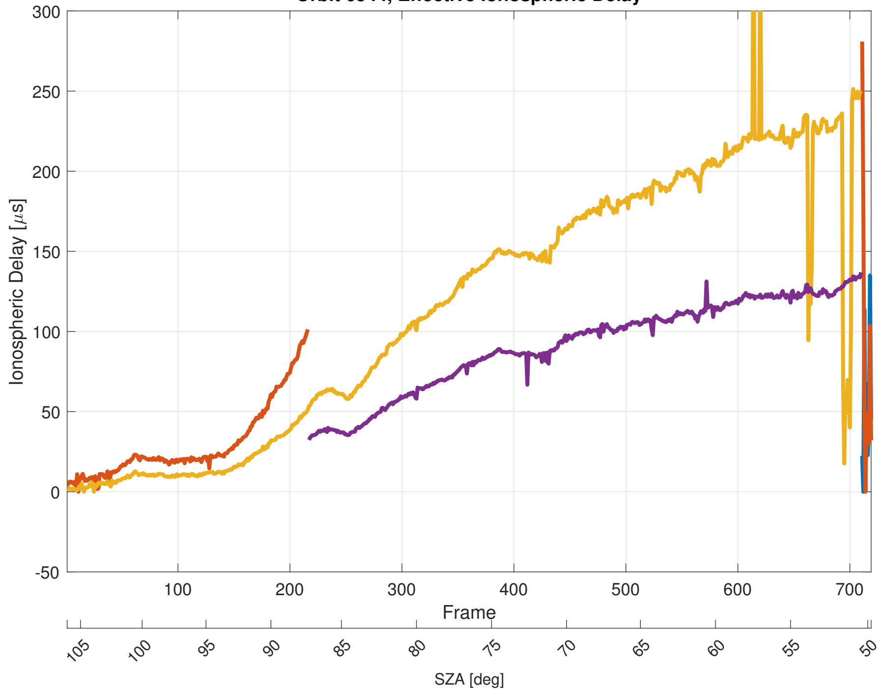
Orbit 6544, Effective Ionospheric Delay
