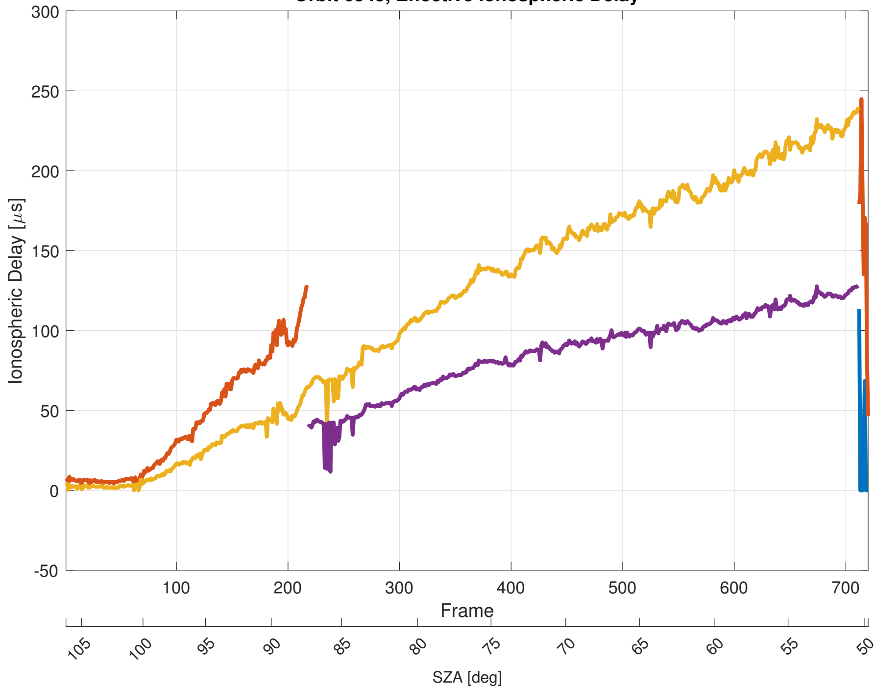
Orbit 6545, Effective Ionospheric Delay
