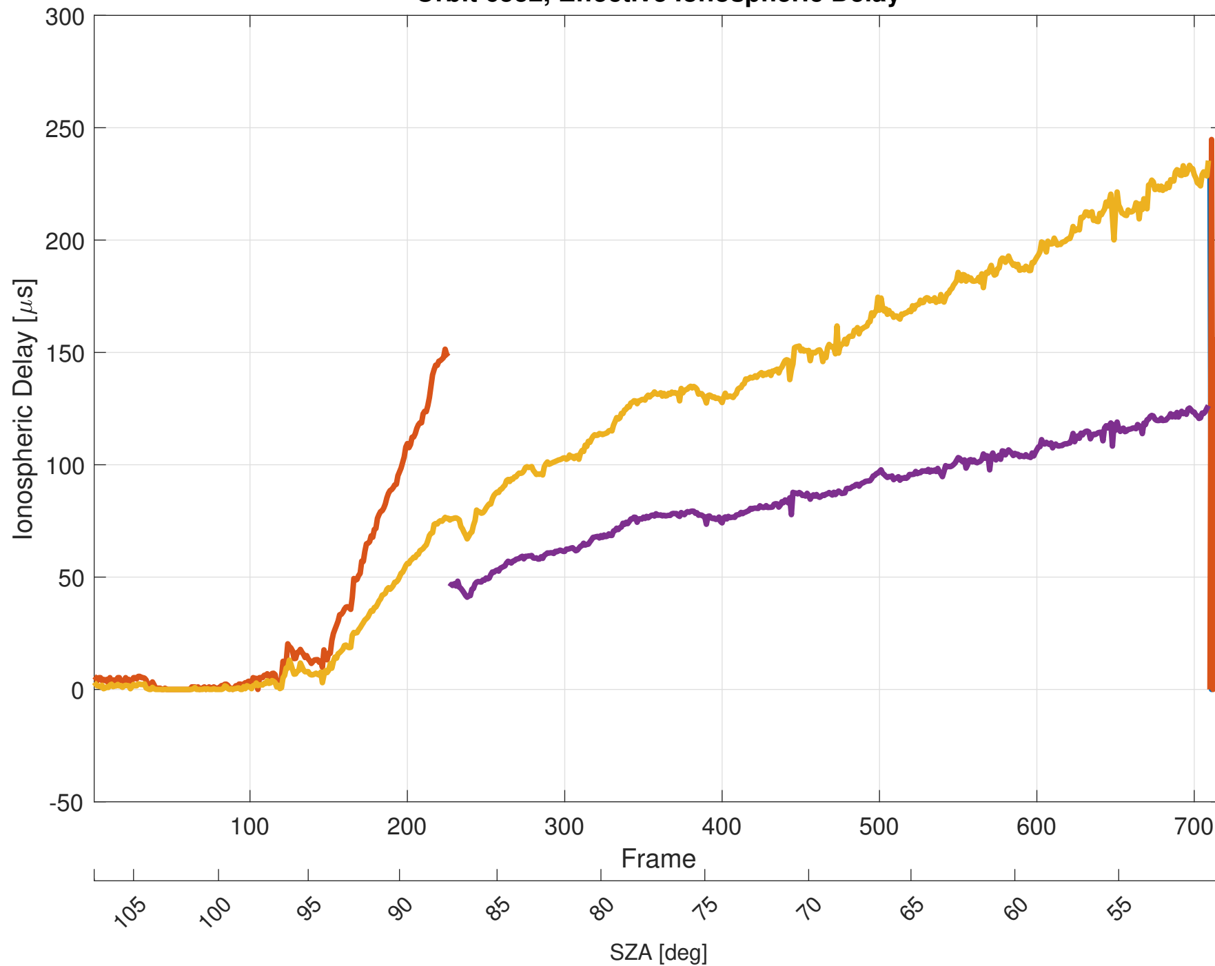
Orbit 6552, Effective Ionospheric Delay
