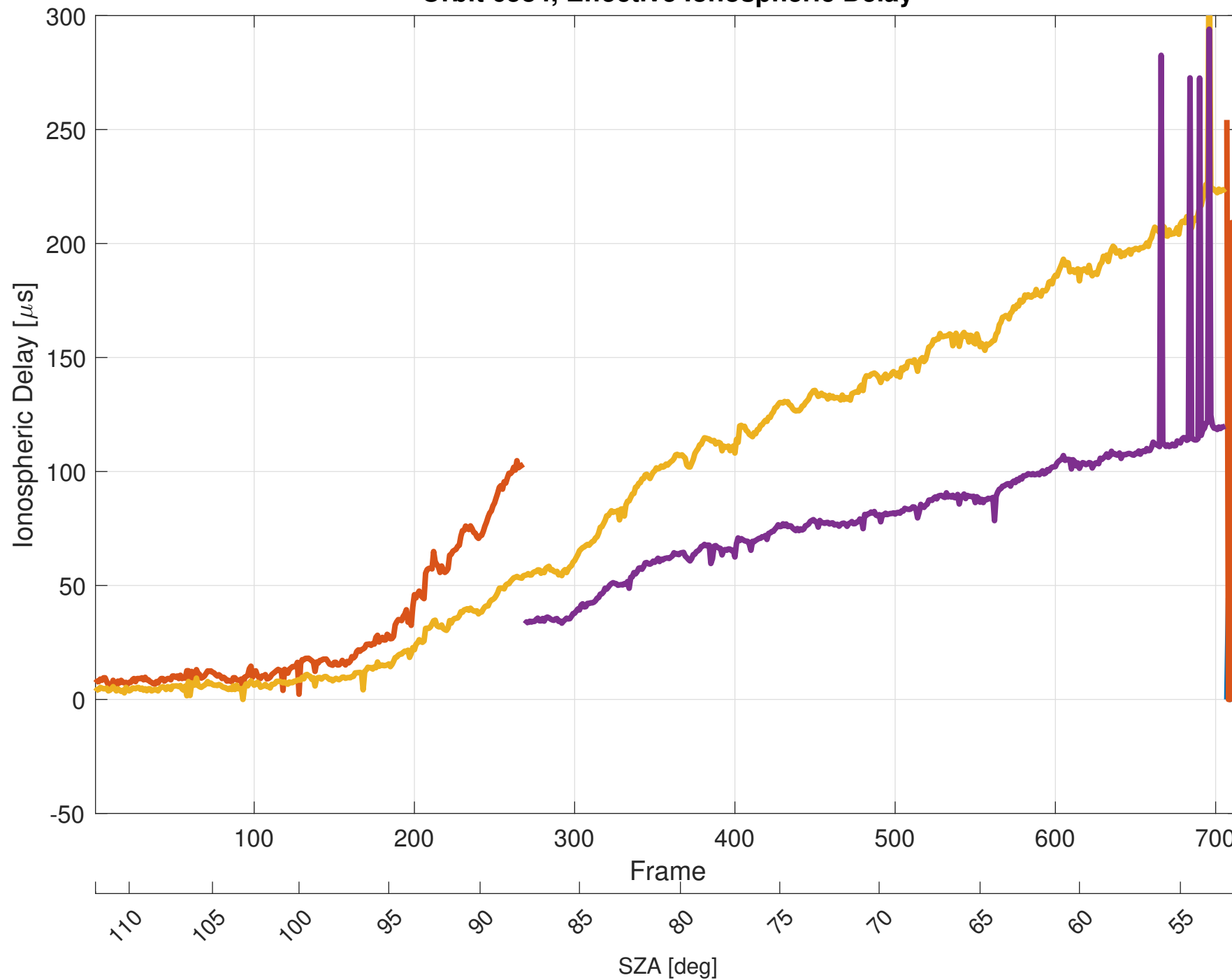
Orbit 6584, Effective Ionospheric Delay
