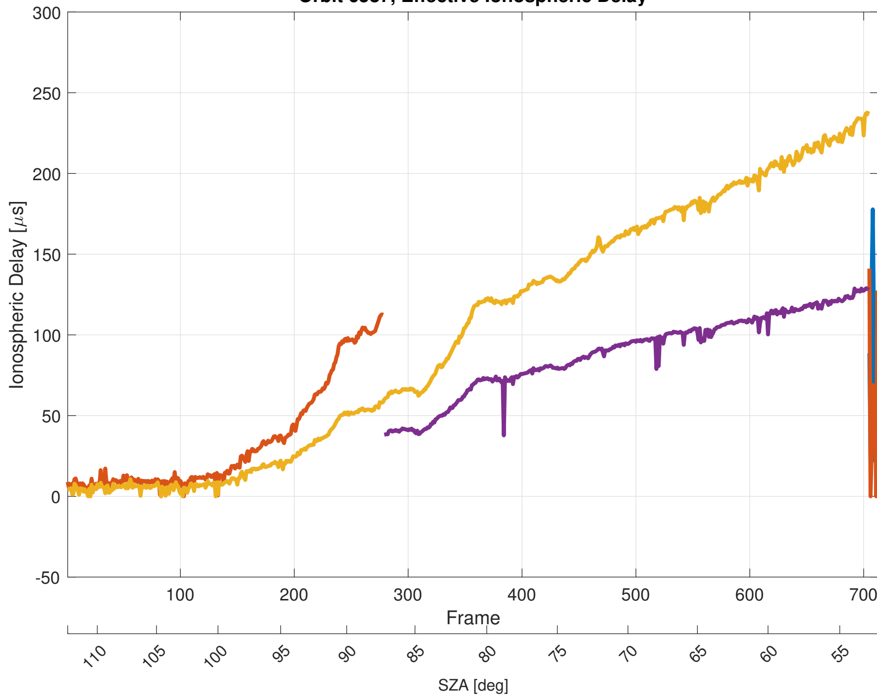
Orbit 6587, Effective Ionospheric Delay
