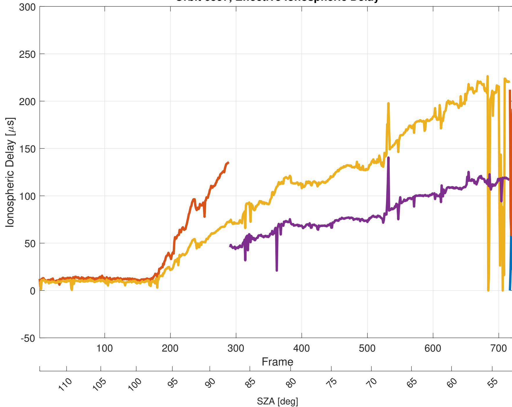
Orbit 6597, Effective Ionospheric Delay
