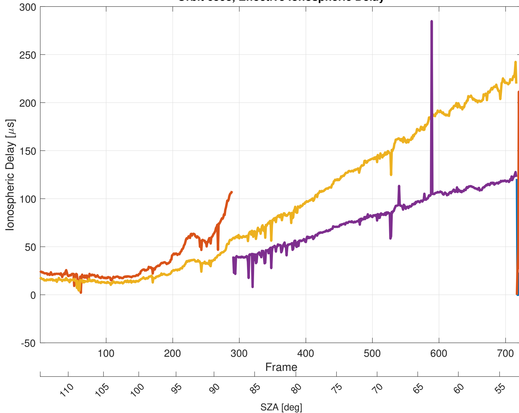
Orbit 6598, Effective Ionospheric Delay
