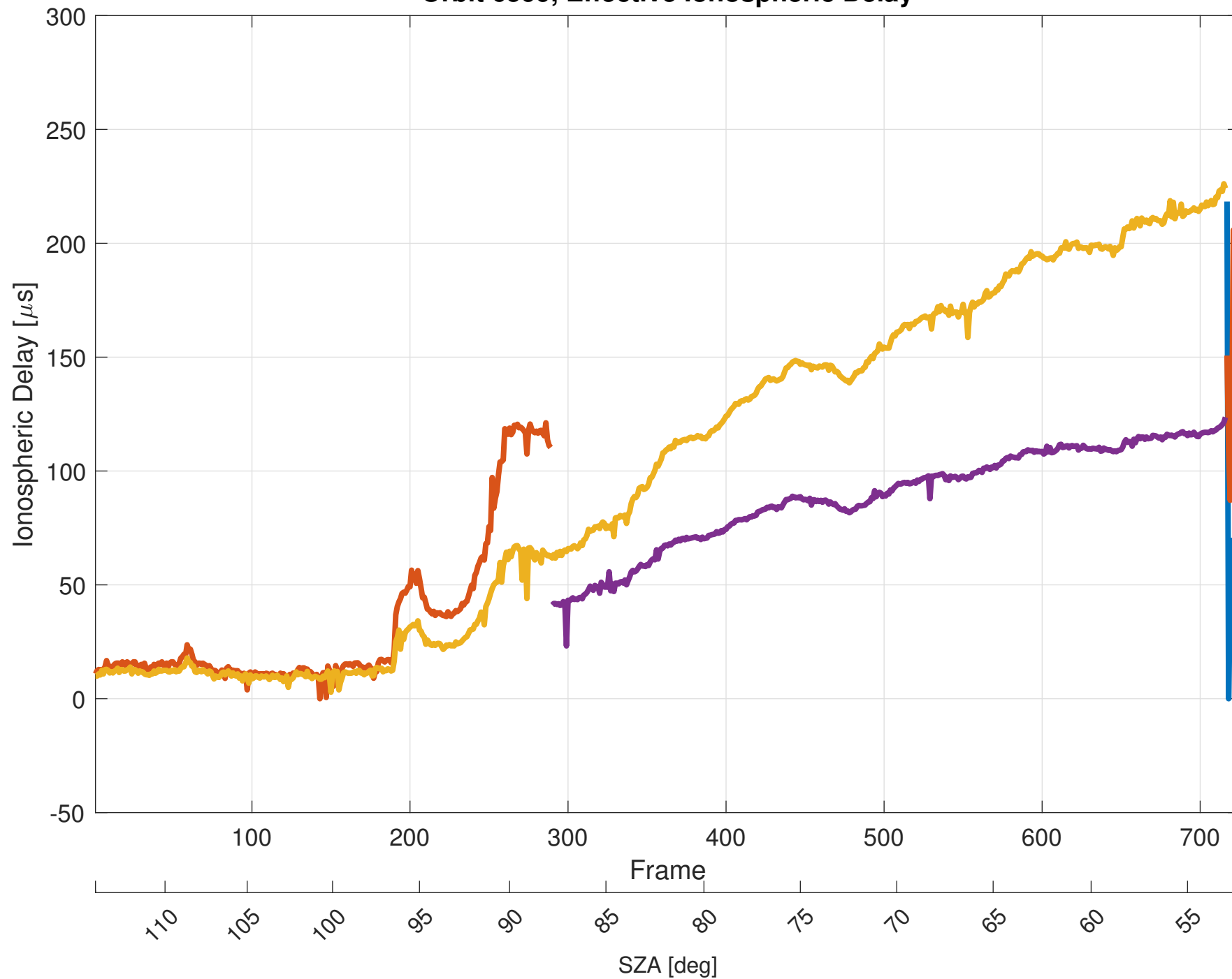
Orbit 6599, Effective Ionospheric Delay
