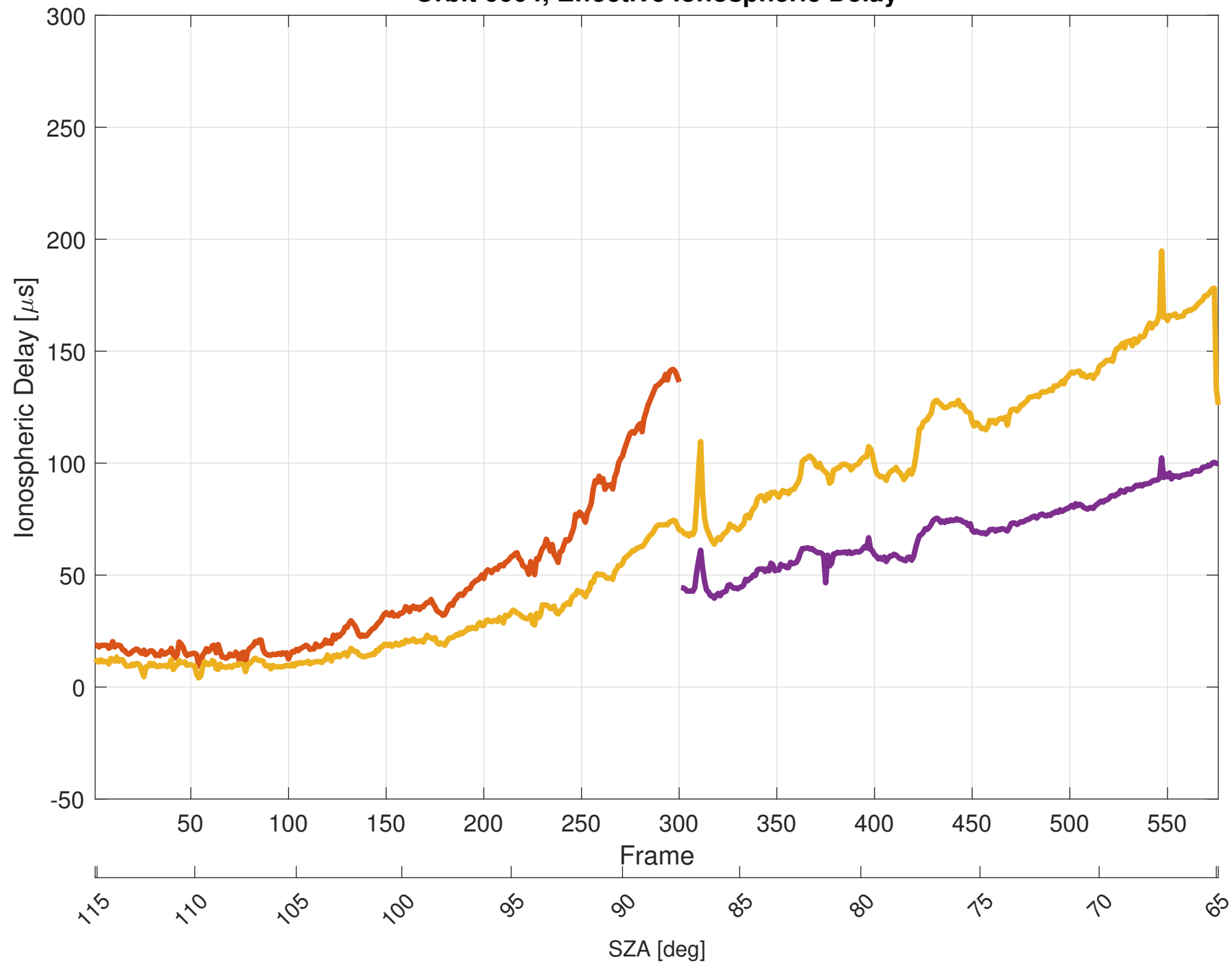
Orbit 6604, Effective Ionospheric Delay
