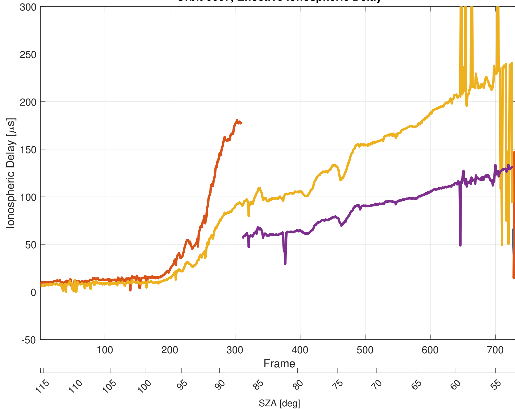
Orbit 6607, Effective Ionospheric Delay
