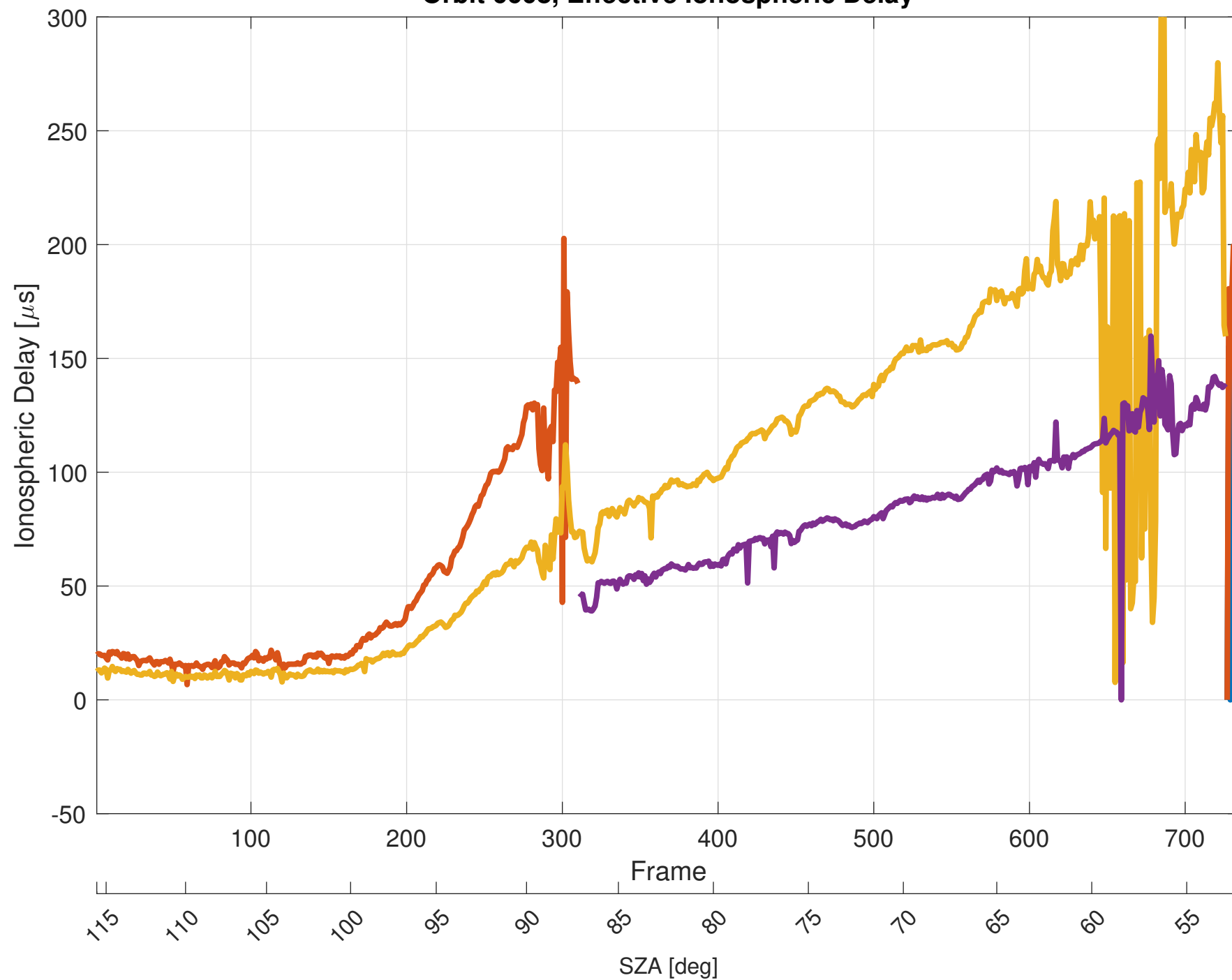
Orbit 6608, Effective Ionospheric Delay
