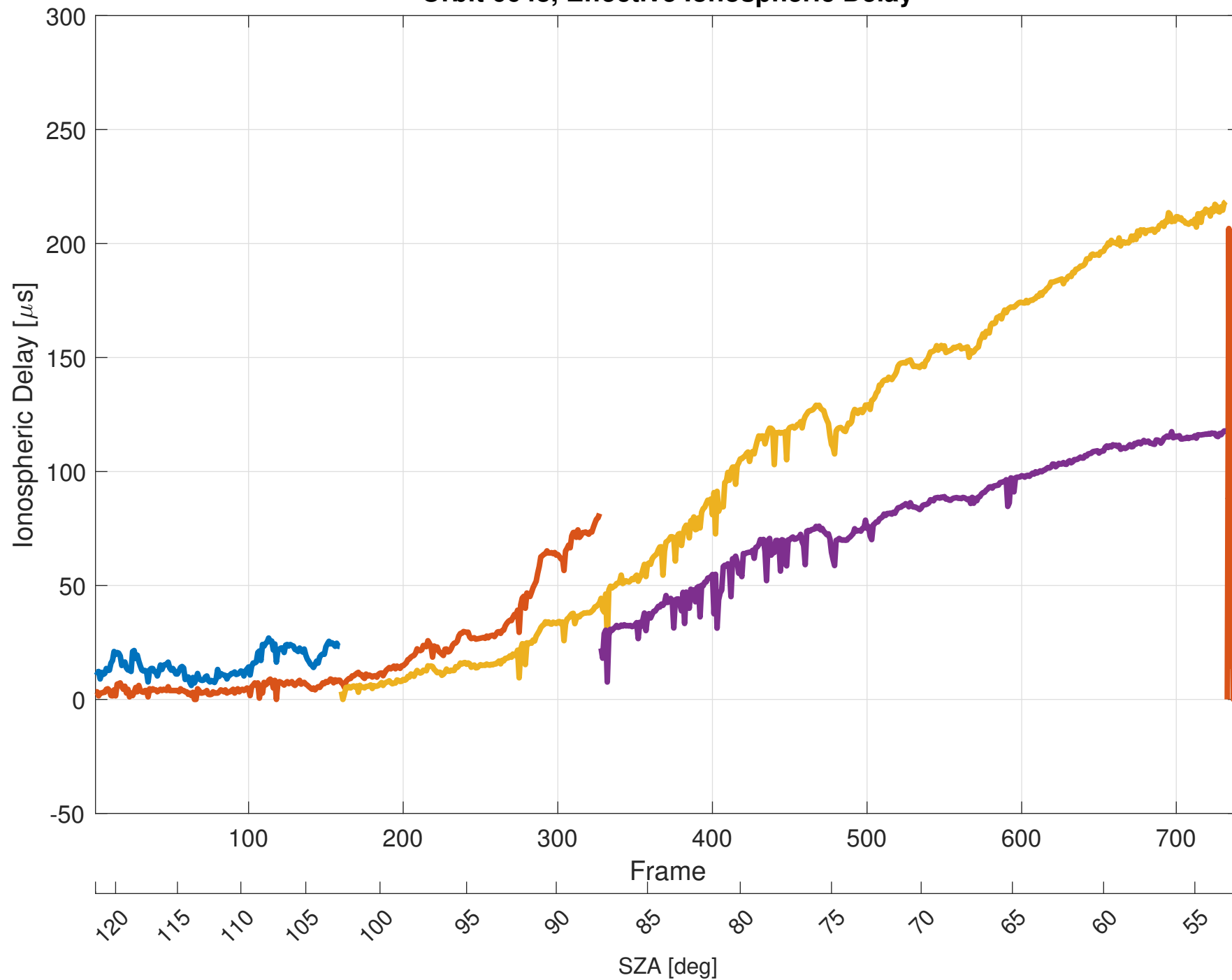
Orbit 6648, Effective Ionospheric Delay
