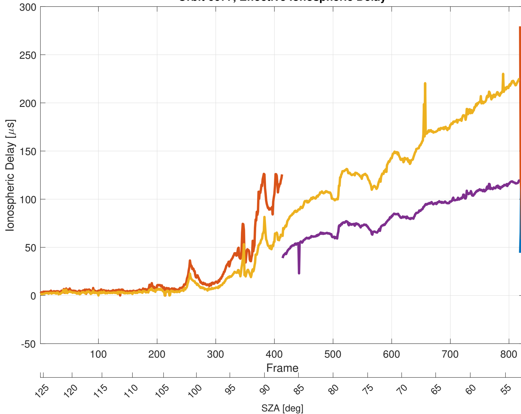
Orbit 6677, Effective Ionospheric Delay
