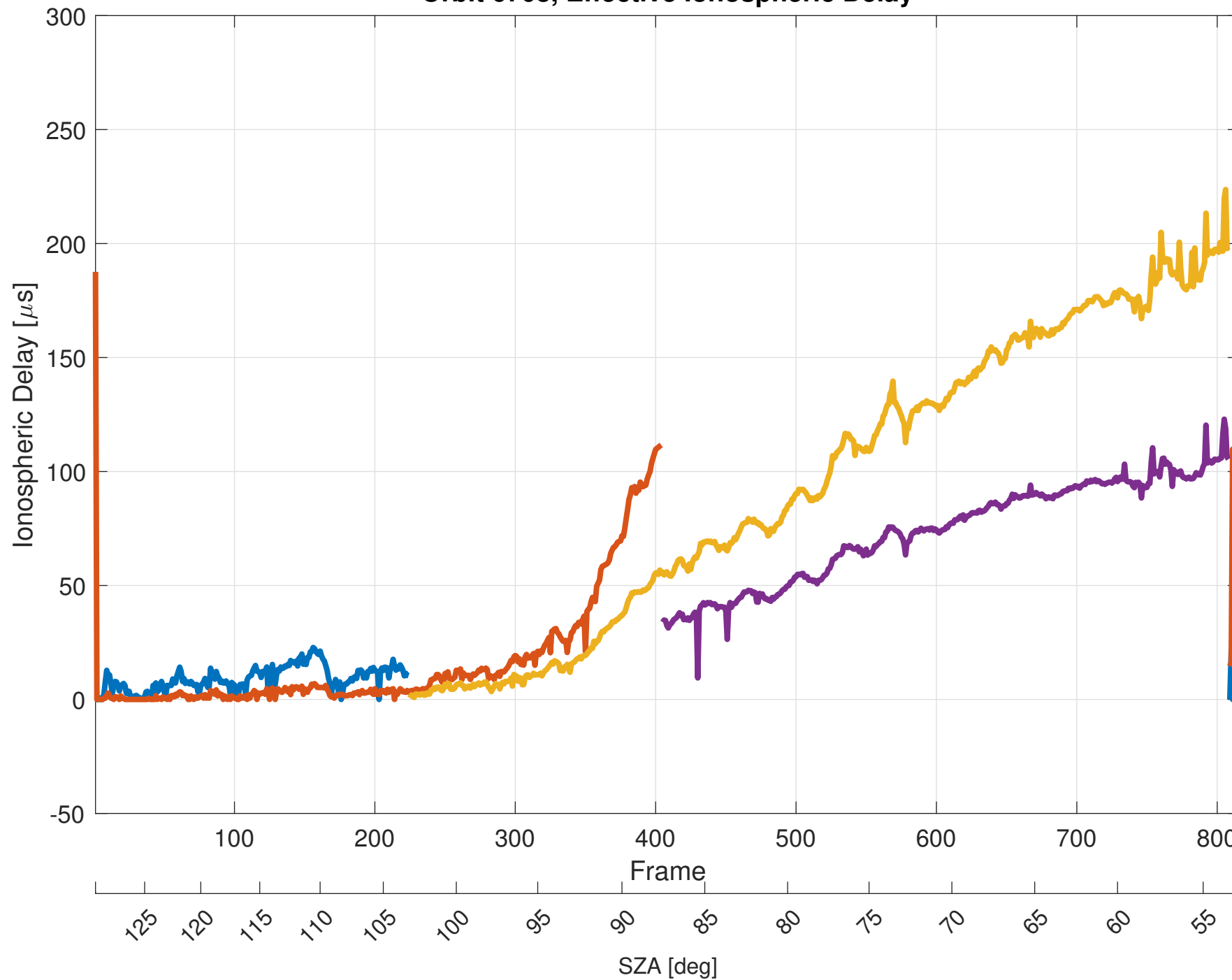
Orbit 6708, Effective Ionospheric Delay
