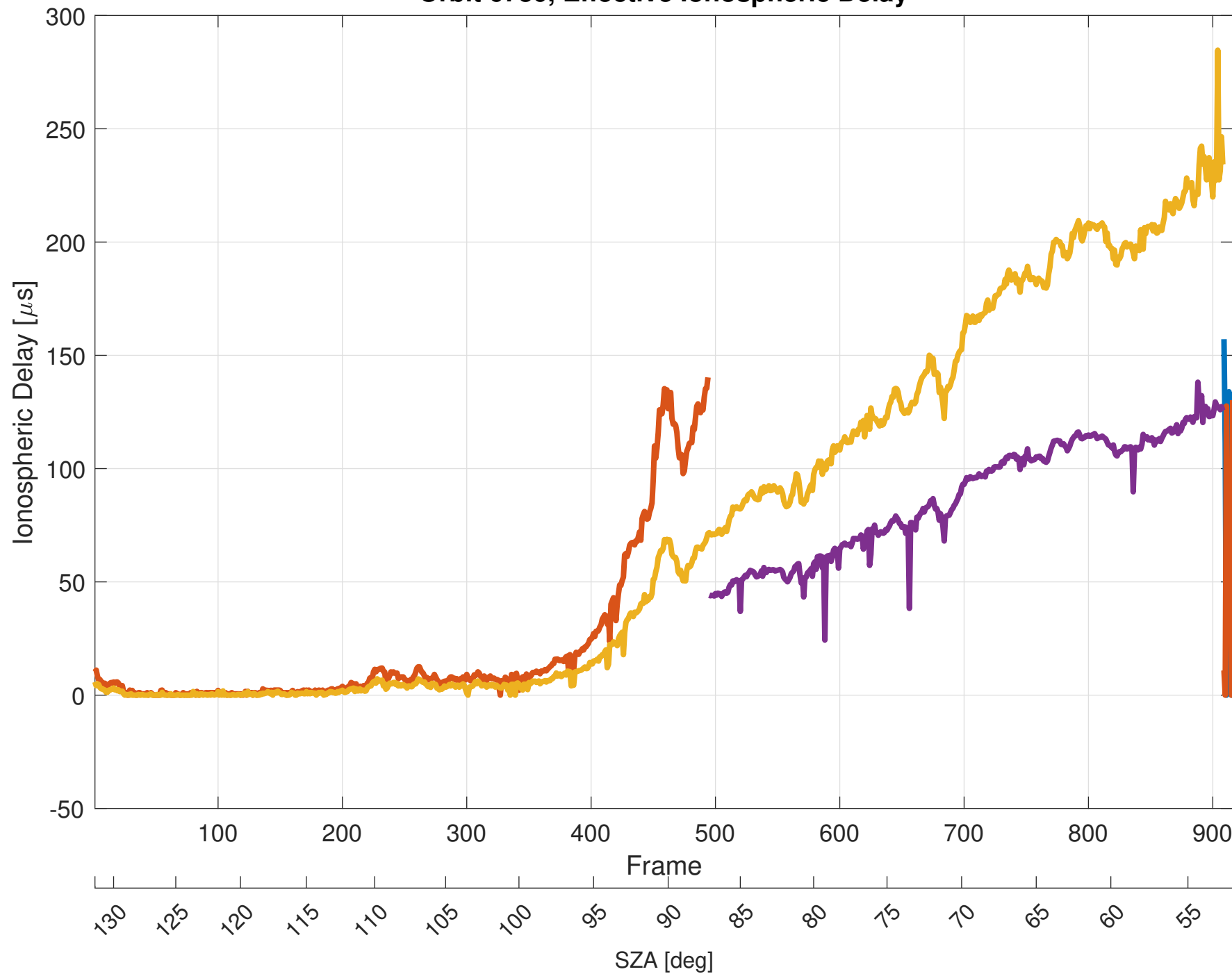
Orbit 6730, Effective Ionospheric Delay
