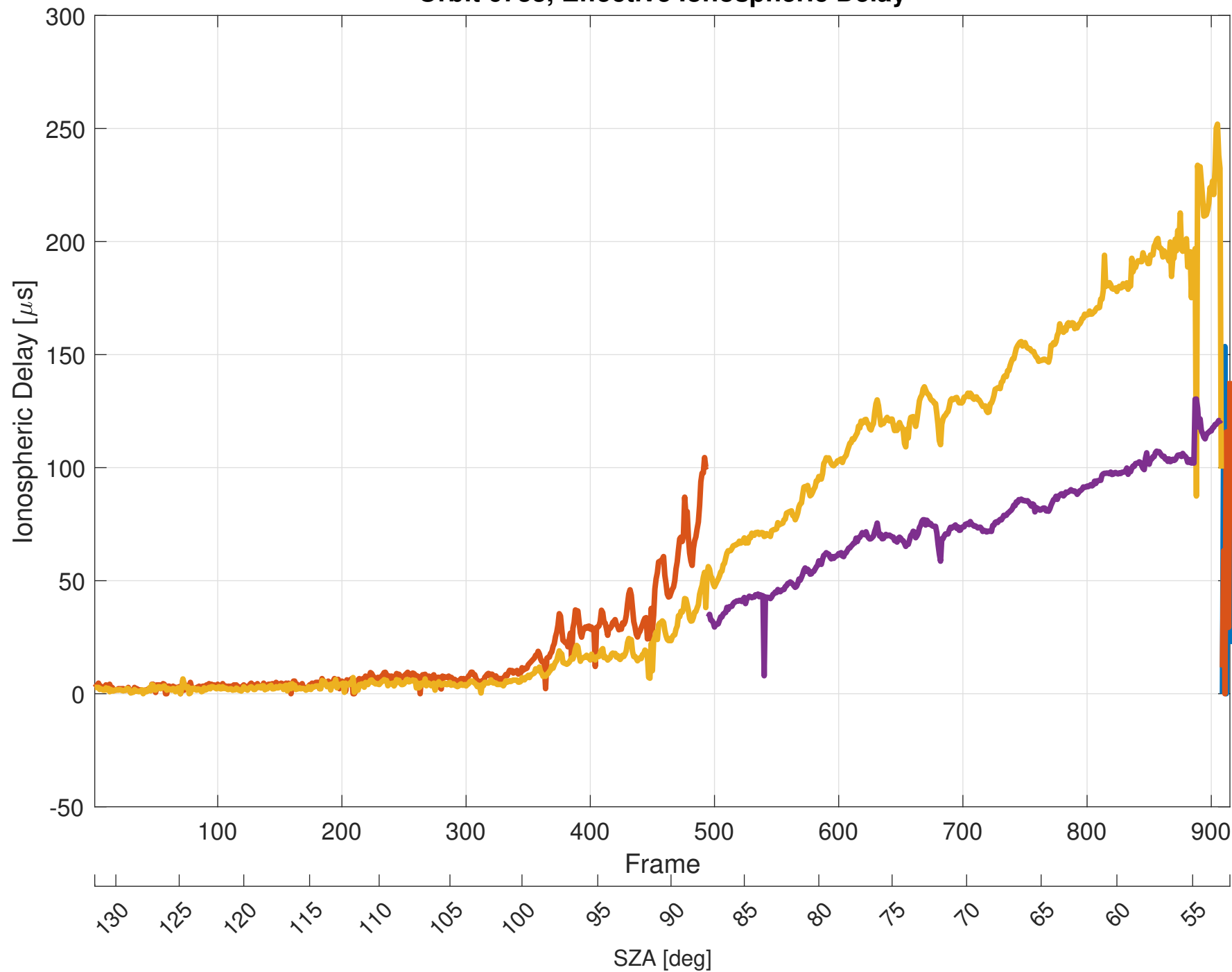
Orbit 6733, Effective Ionospheric Delay
