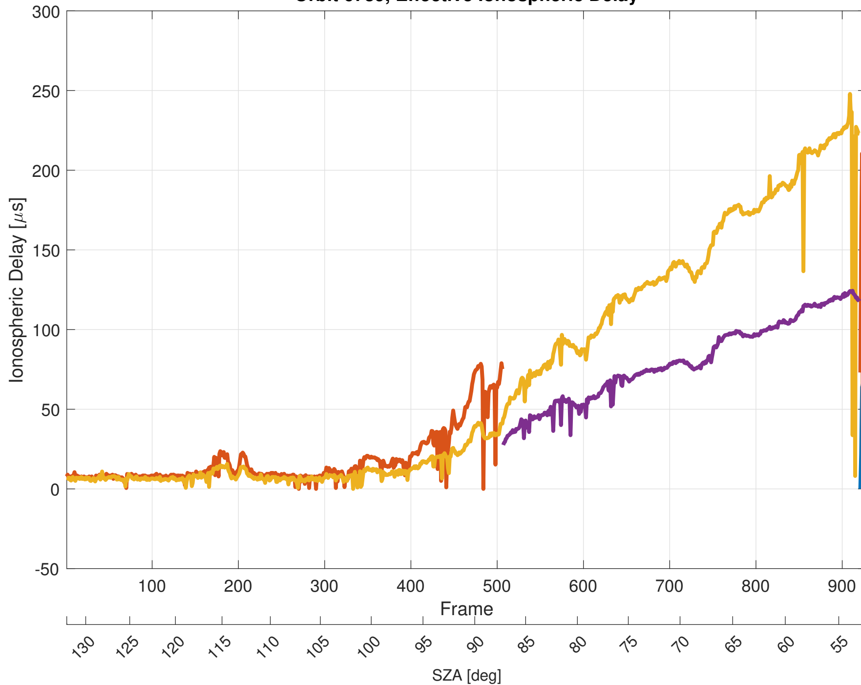
Orbit 6739, Effective Ionospheric Delay
