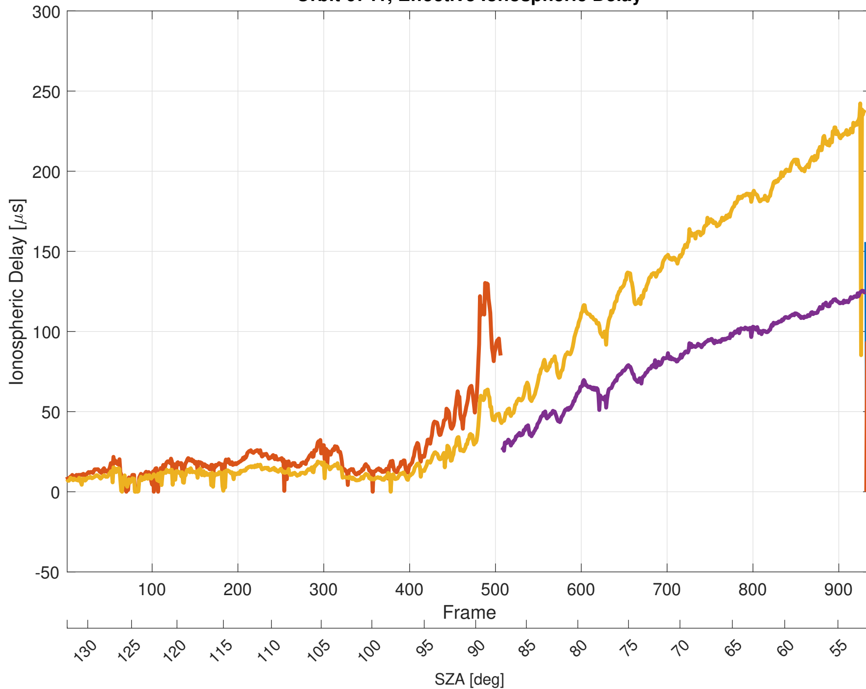
Orbit 6741, Effective Ionospheric Delay
