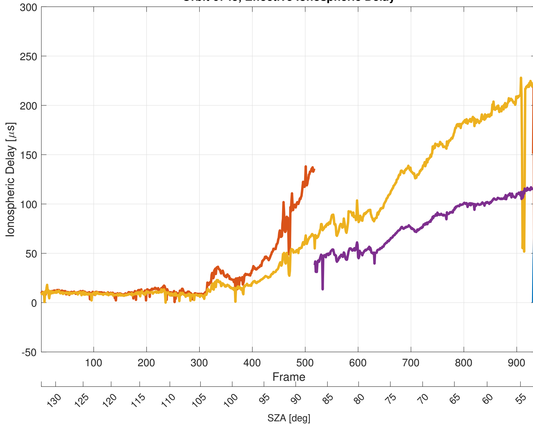
Orbit 6745, Effective Ionospheric Delay
