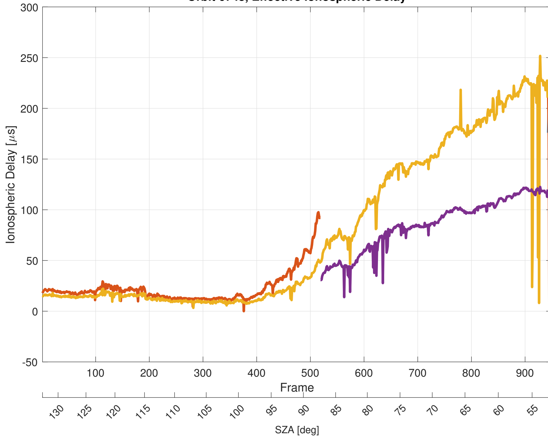
Orbit 6748, Effective Ionospheric Delay
