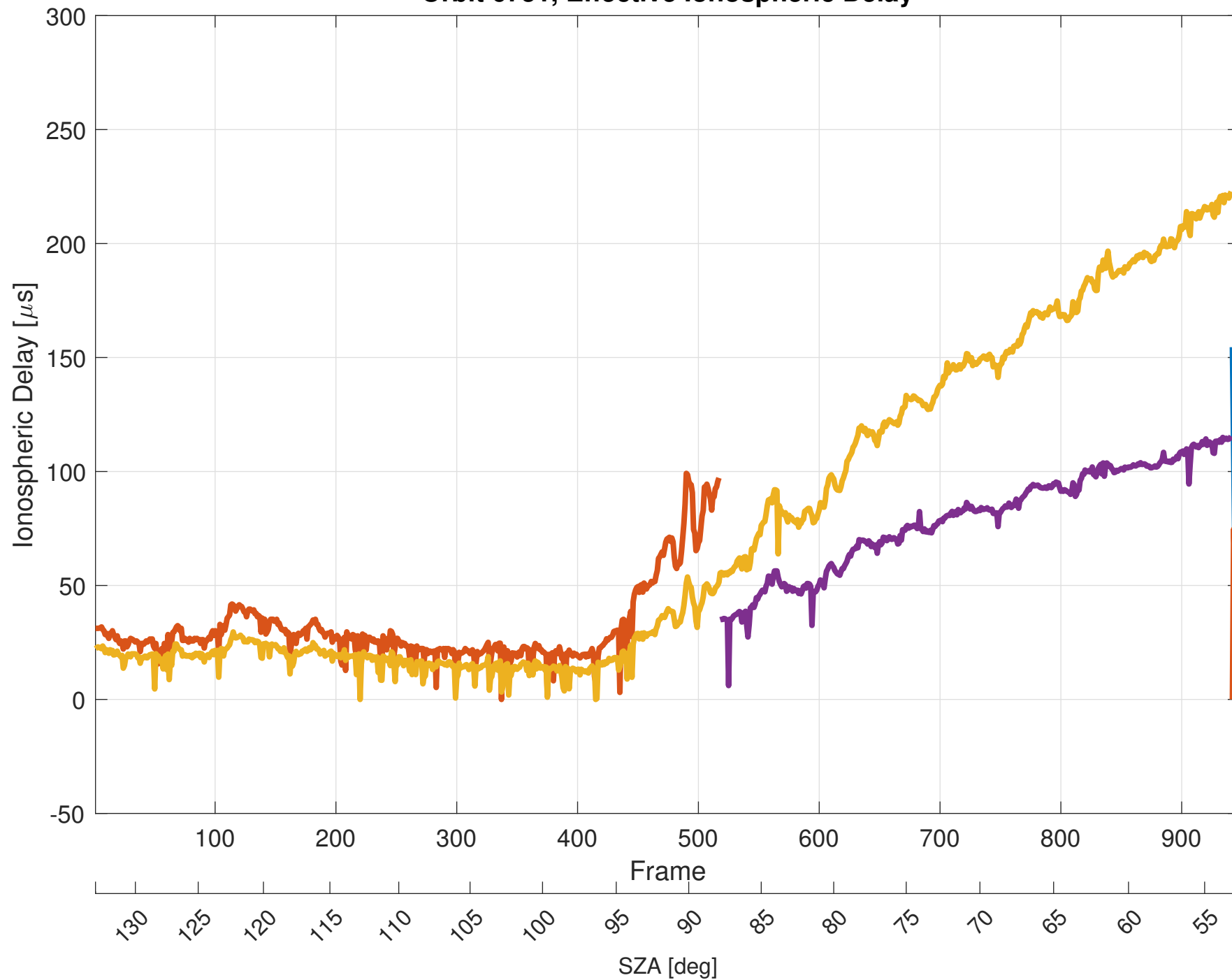
Orbit 6751, Effective Ionospheric Delay
