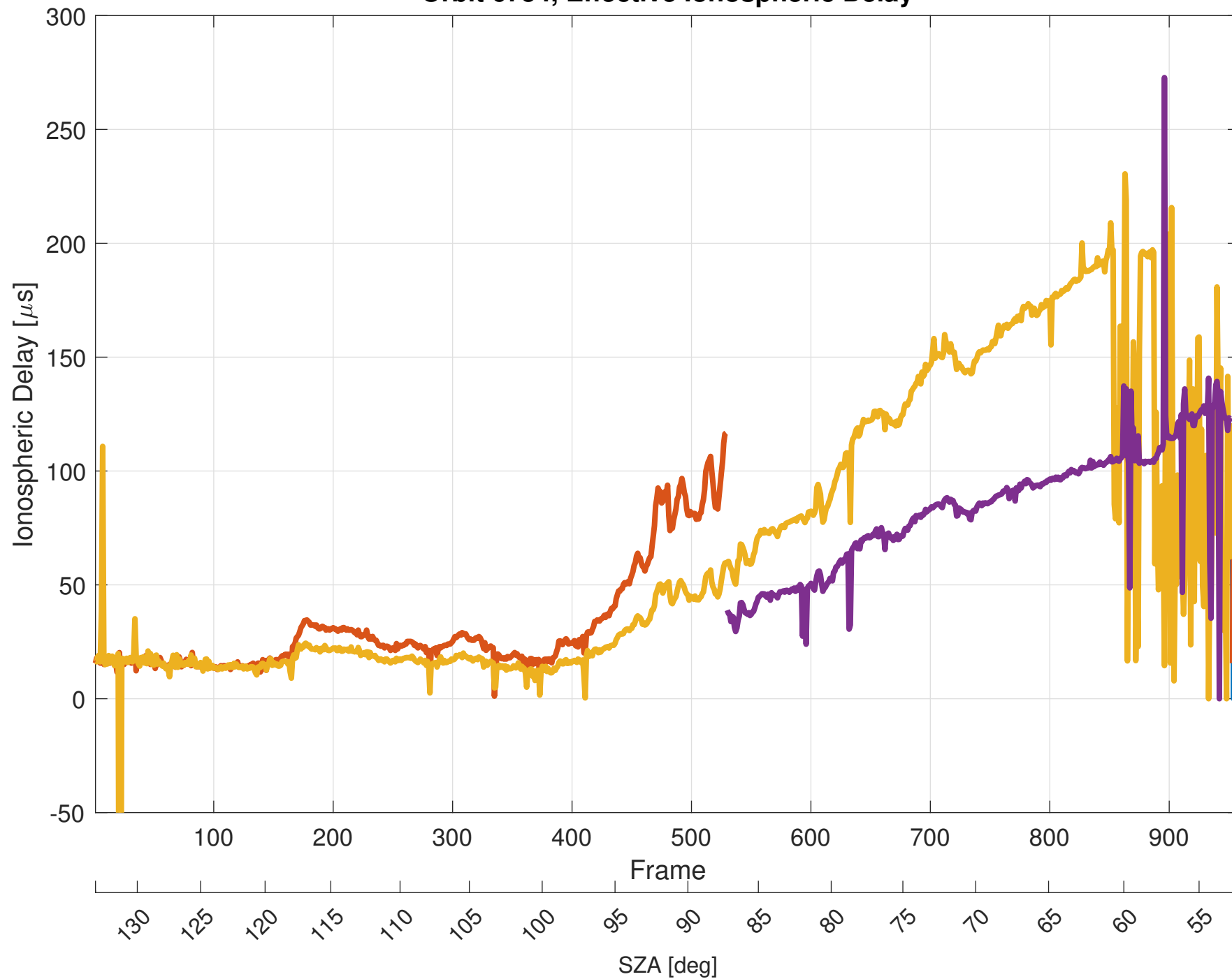
Orbit 6754, Effective Ionospheric Delay
