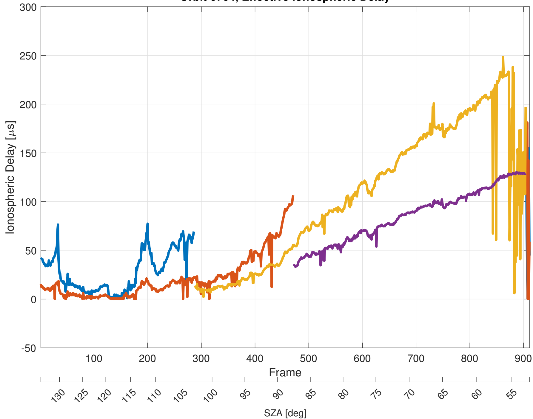
Orbit 6764, Effective Ionospheric Delay
