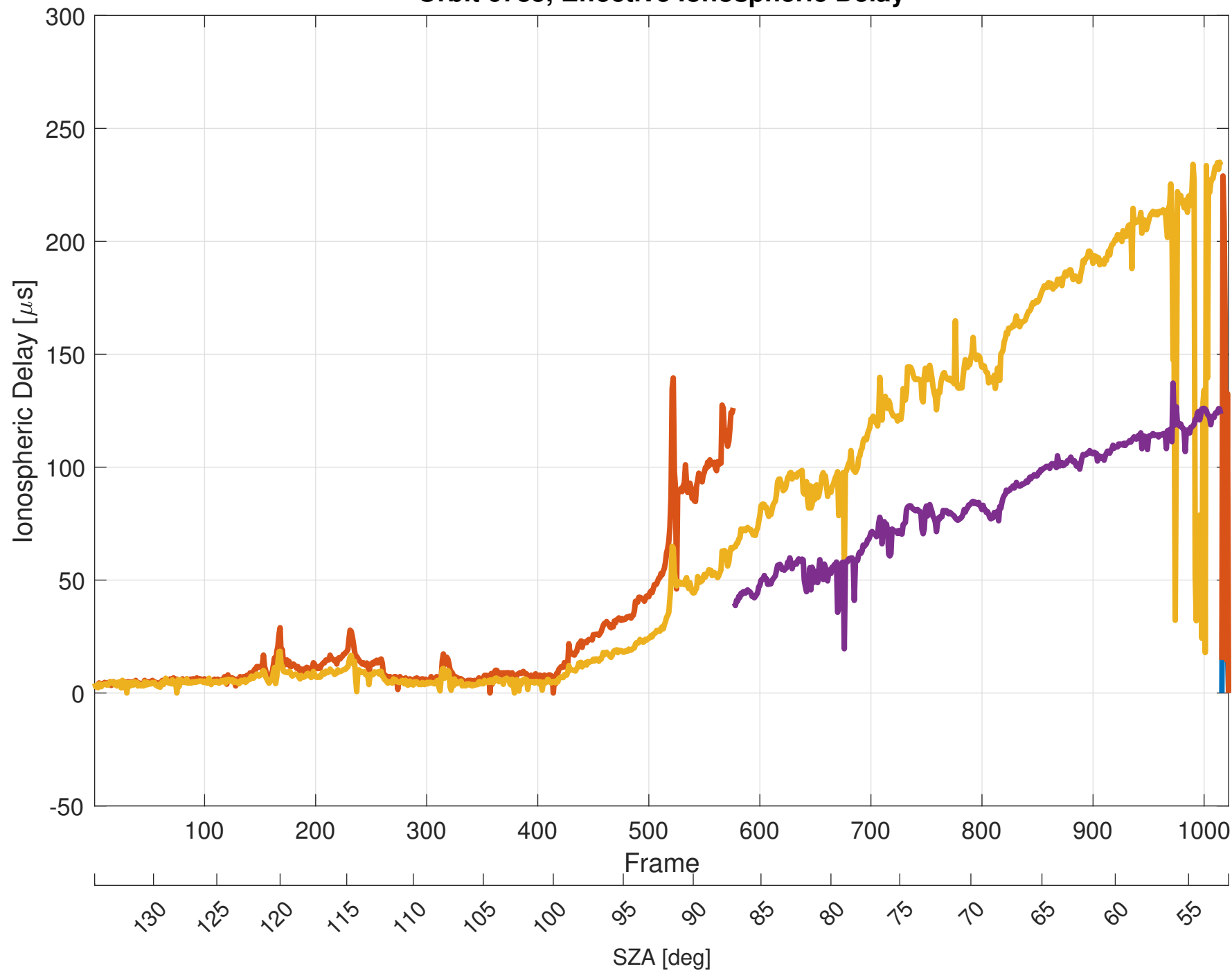
Orbit 6785, Effective Ionospheric Delay
