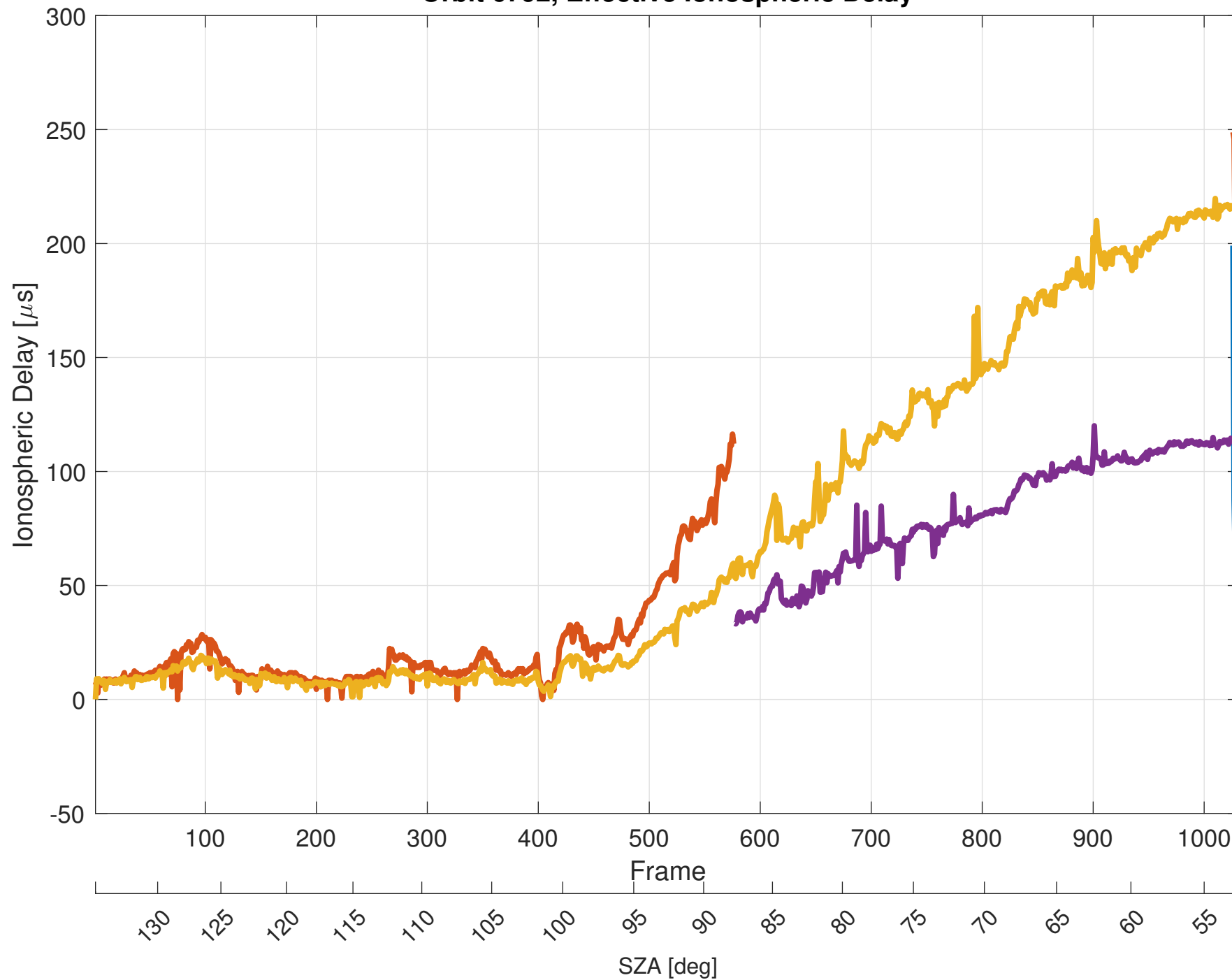
Orbit 6792, Effective Ionospheric Delay
