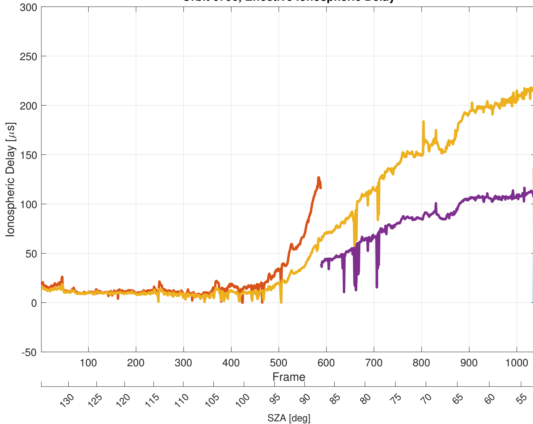
Orbit 6796, Effective Ionospheric Delay
