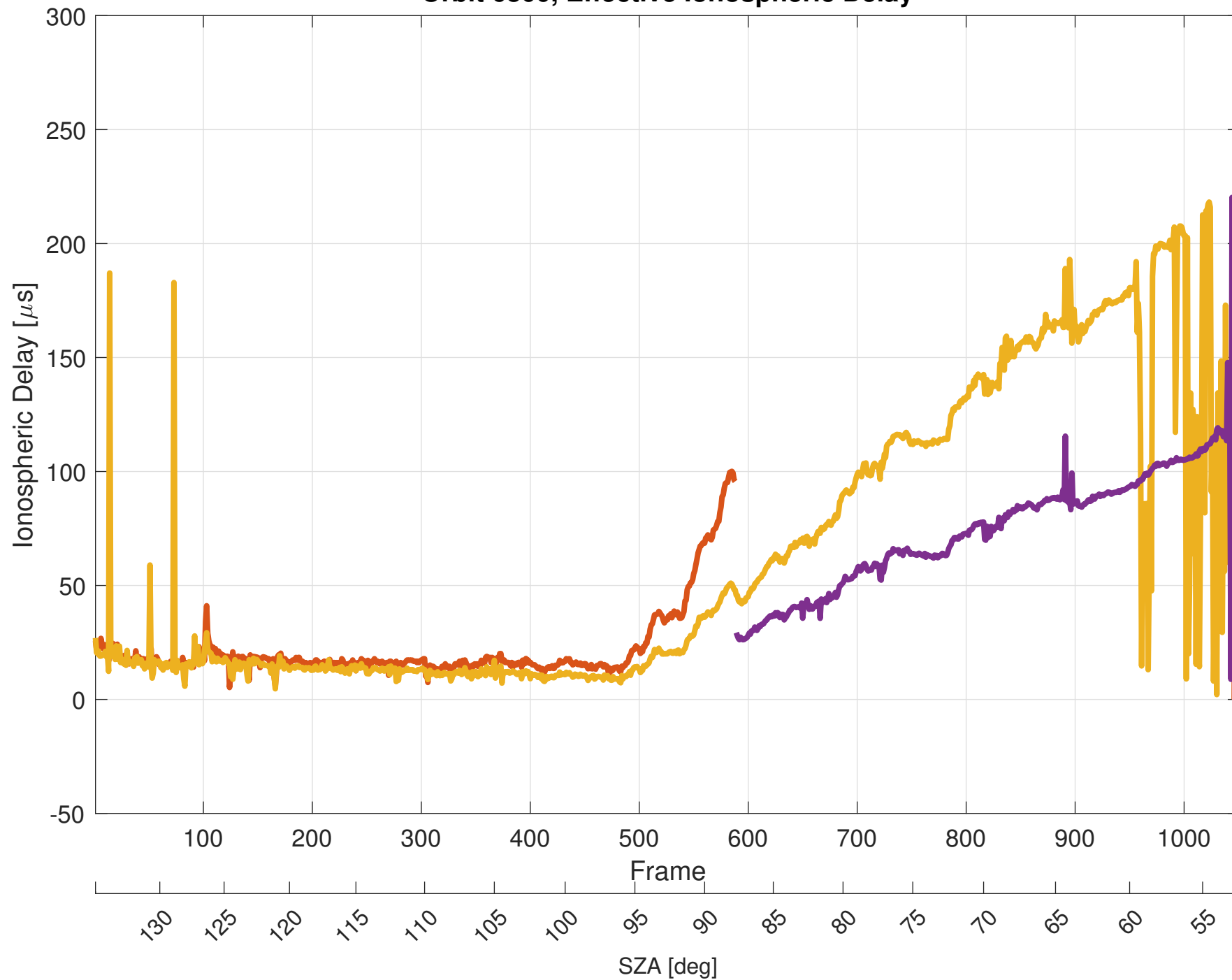
Orbit 6800, Effective Ionospheric Delay
