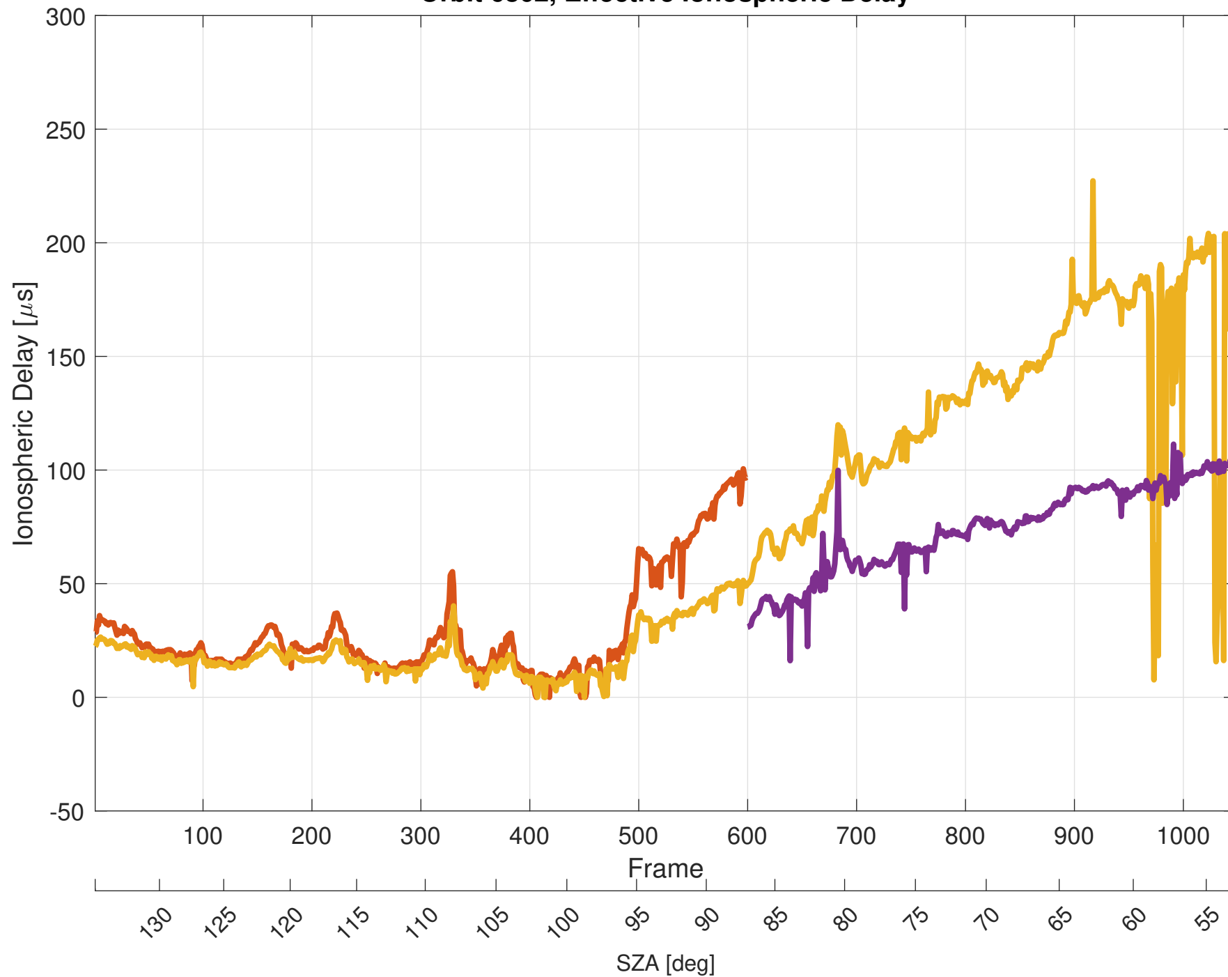
Orbit 6802, Effective Ionospheric Delay
