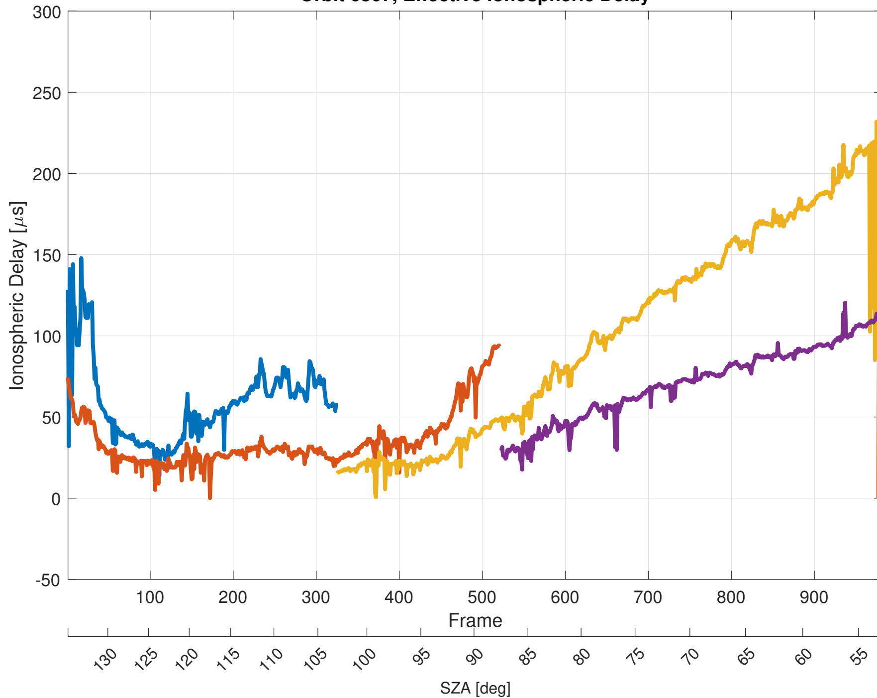
Orbit 6807, Effective Ionospheric Delay
