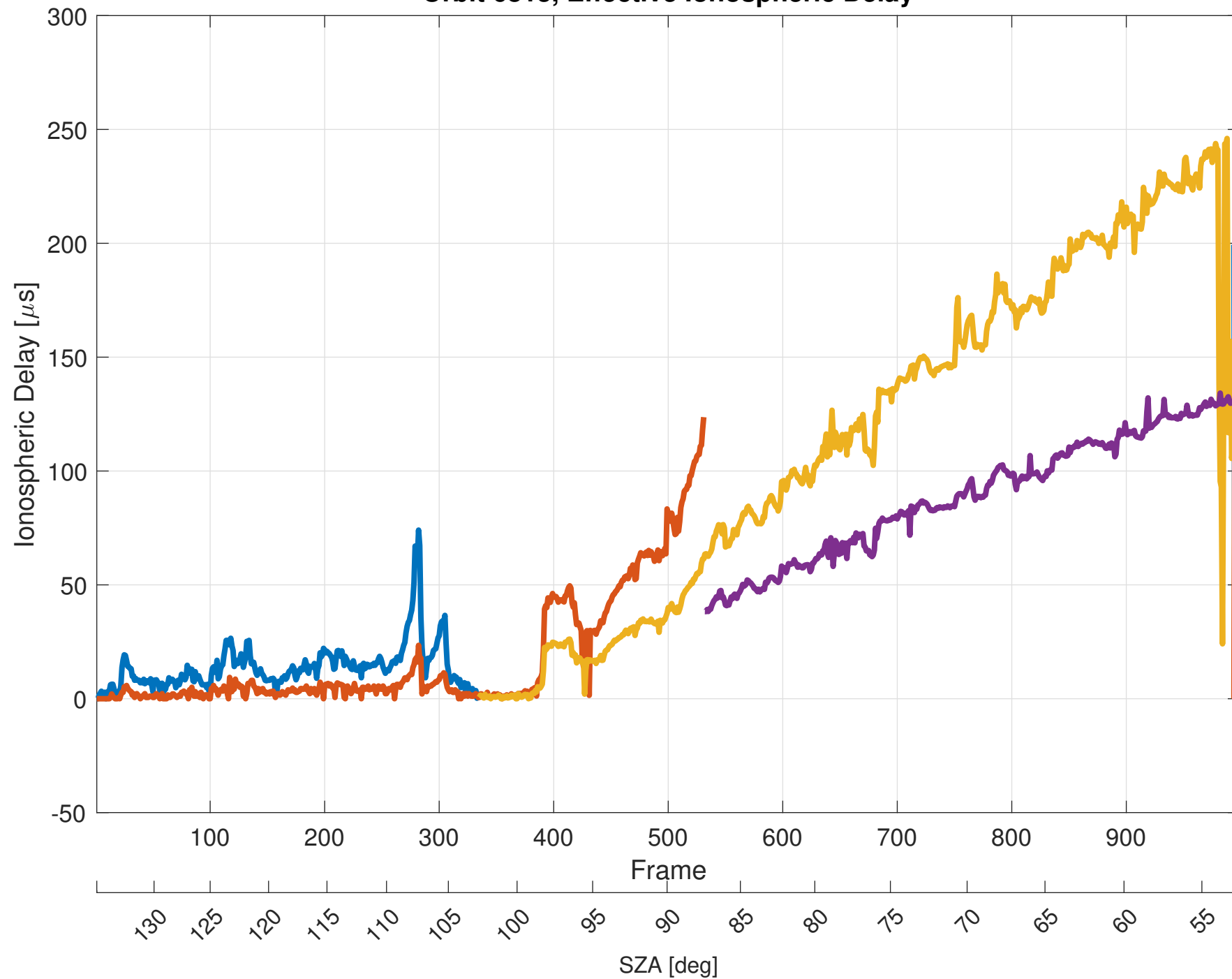
Orbit 6813, Effective Ionospheric Delay
