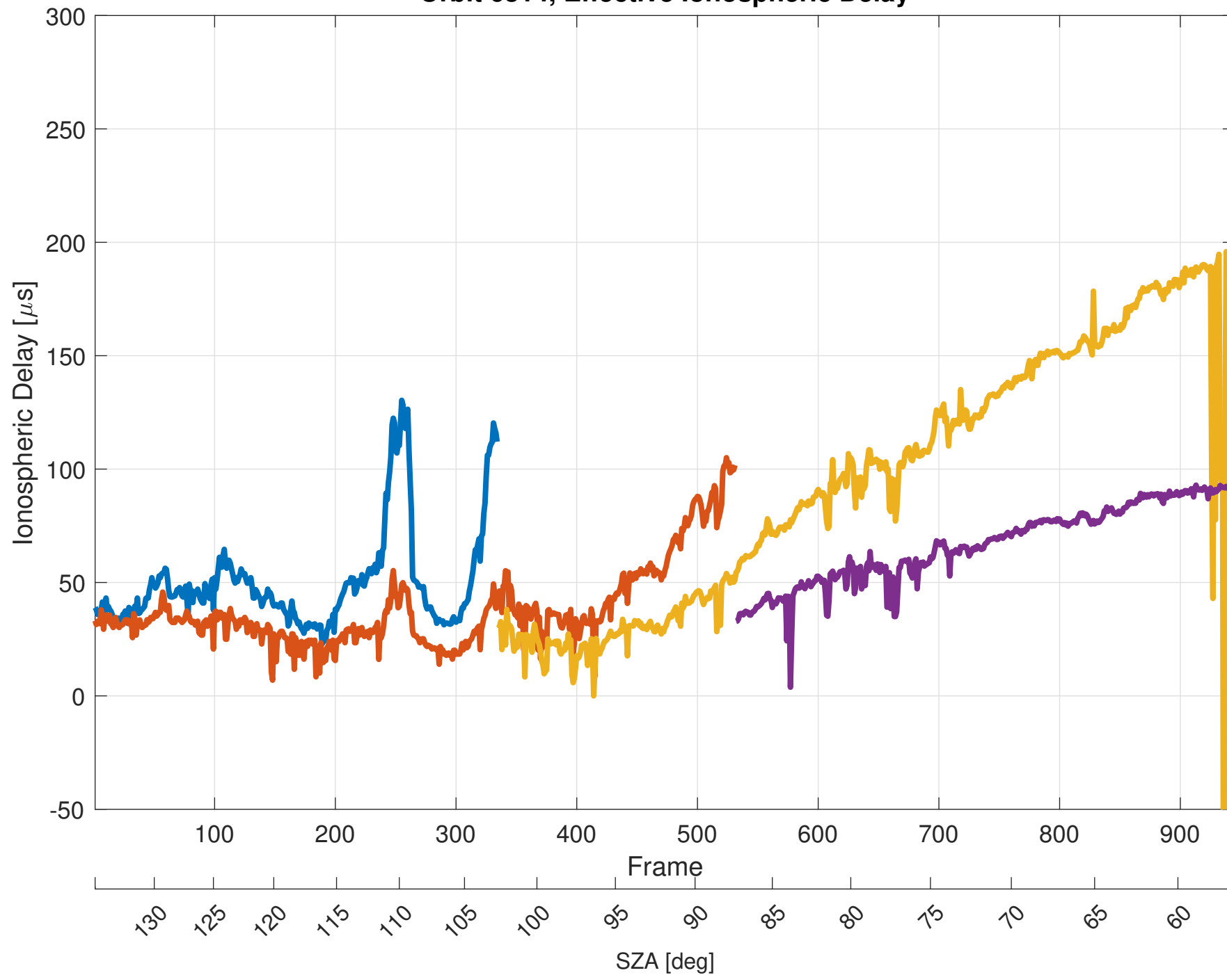
Orbit 6814, Effective Ionospheric Delay
