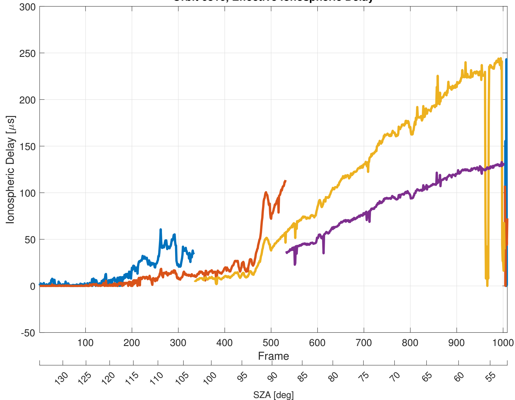
Orbit 6816, Effective Ionospheric Delay
