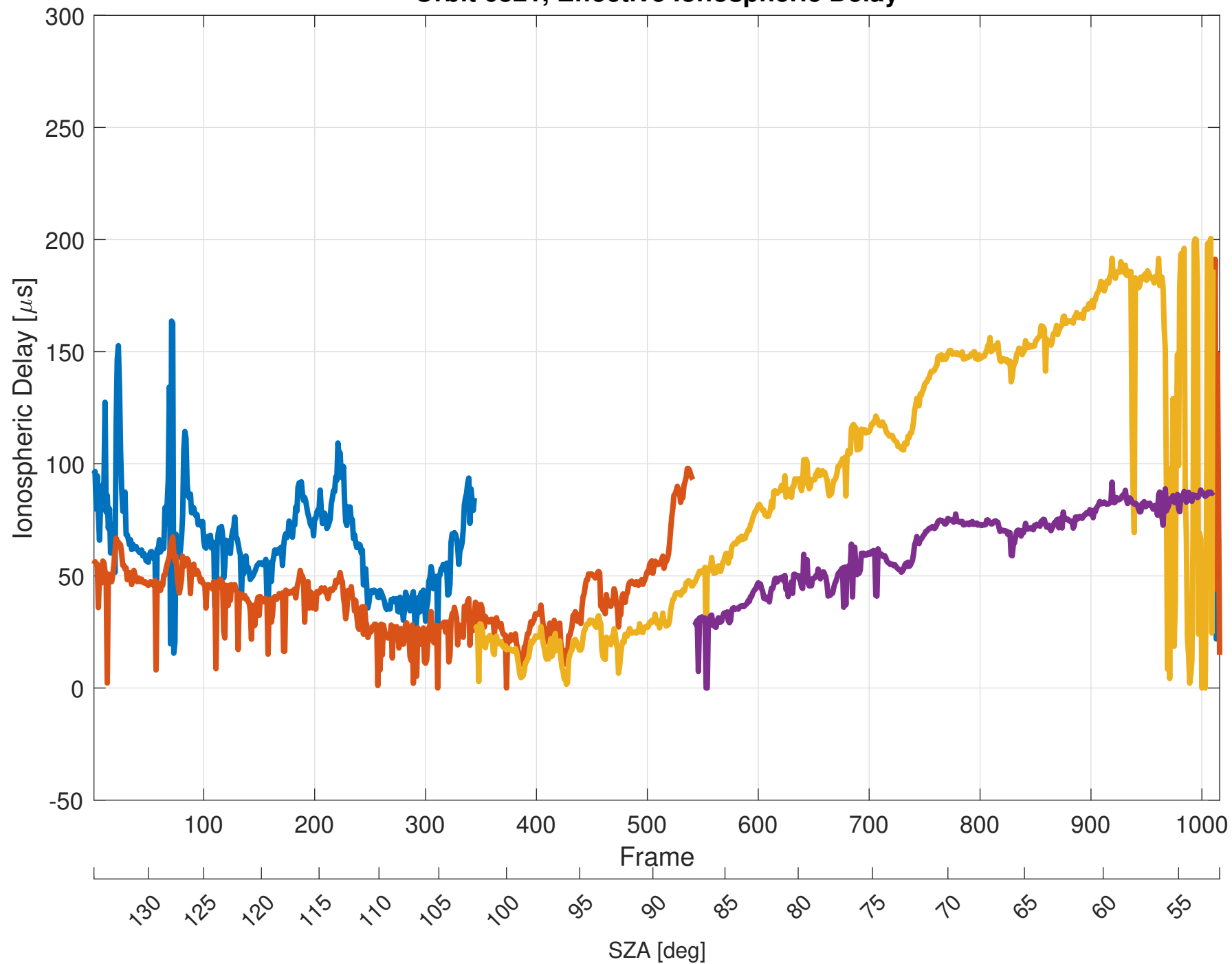
Orbit 6821, Effective Ionospheric Delay
