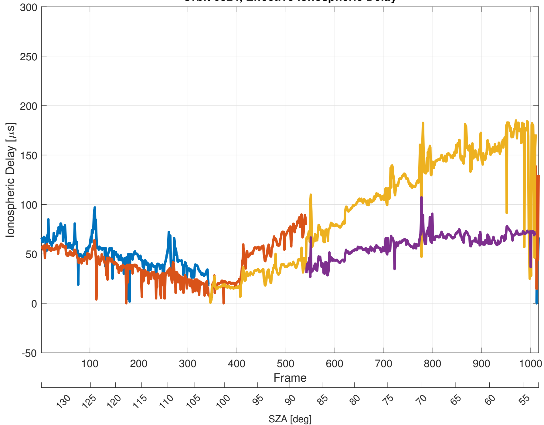
Orbit 6824, Effective Ionospheric Delay
