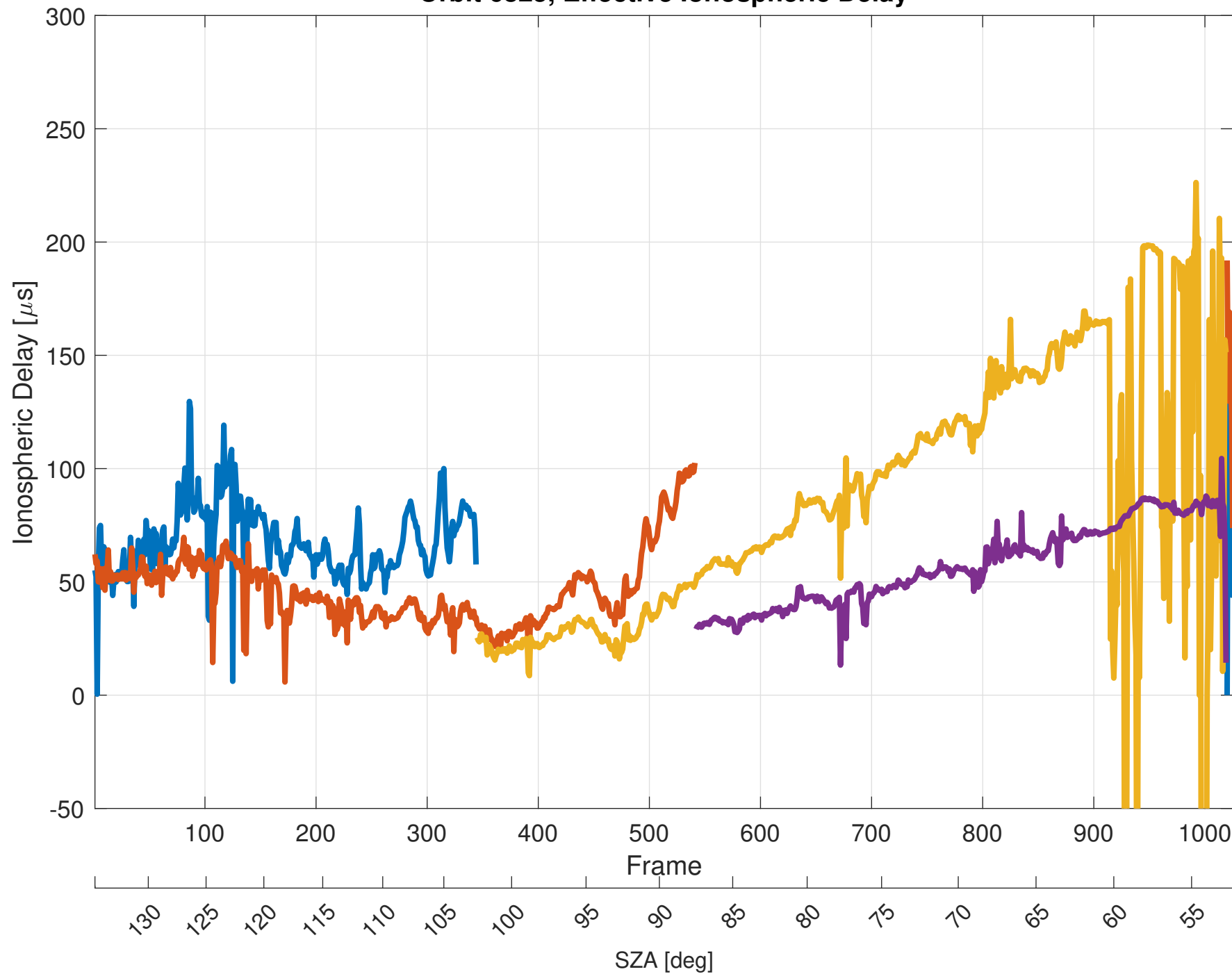
Orbit 6825, Effective Ionospheric Delay
