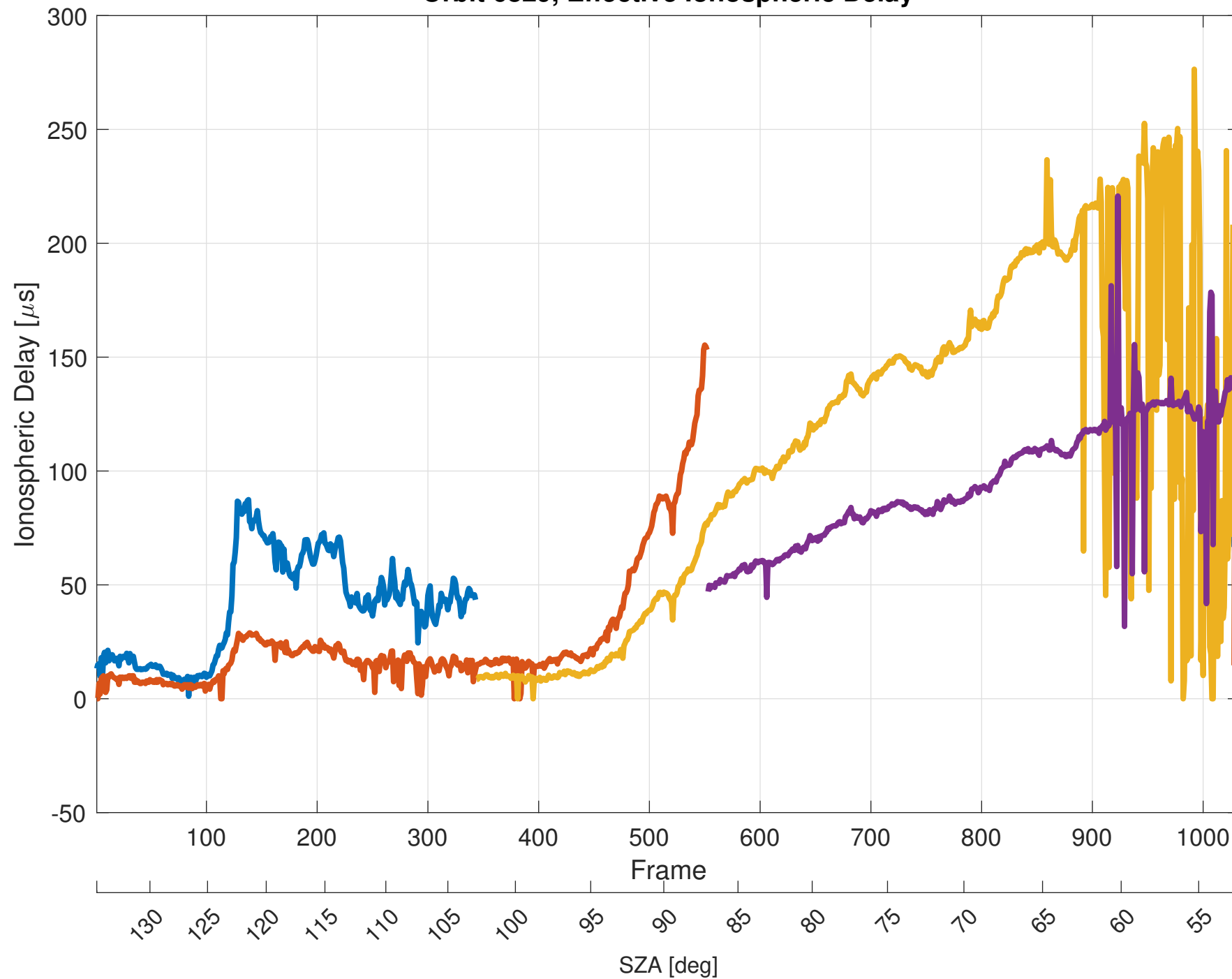
Orbit 6829, Effective Ionospheric Delay
