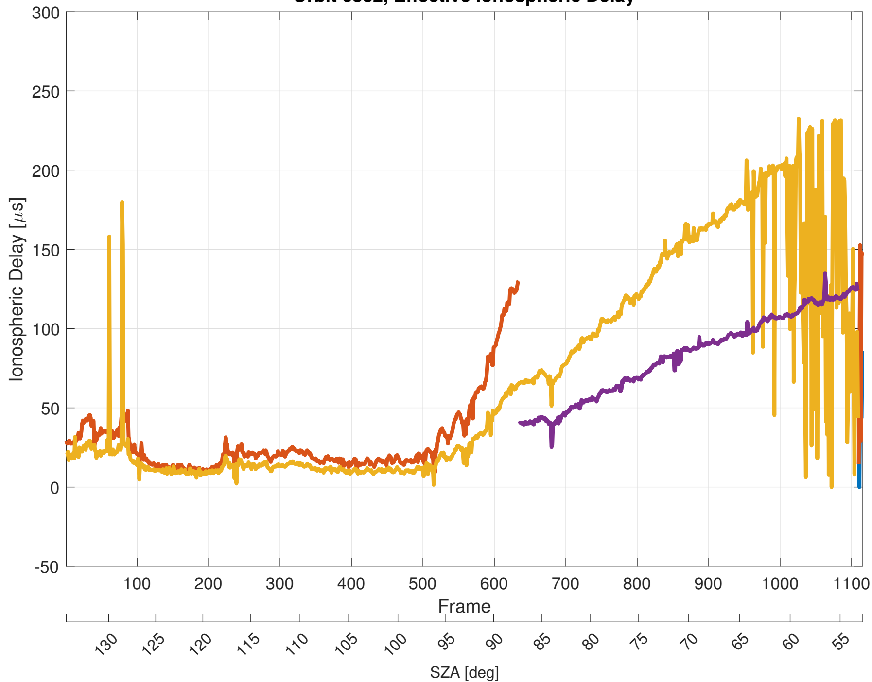
Orbit 6832, Effective Ionospheric Delay
