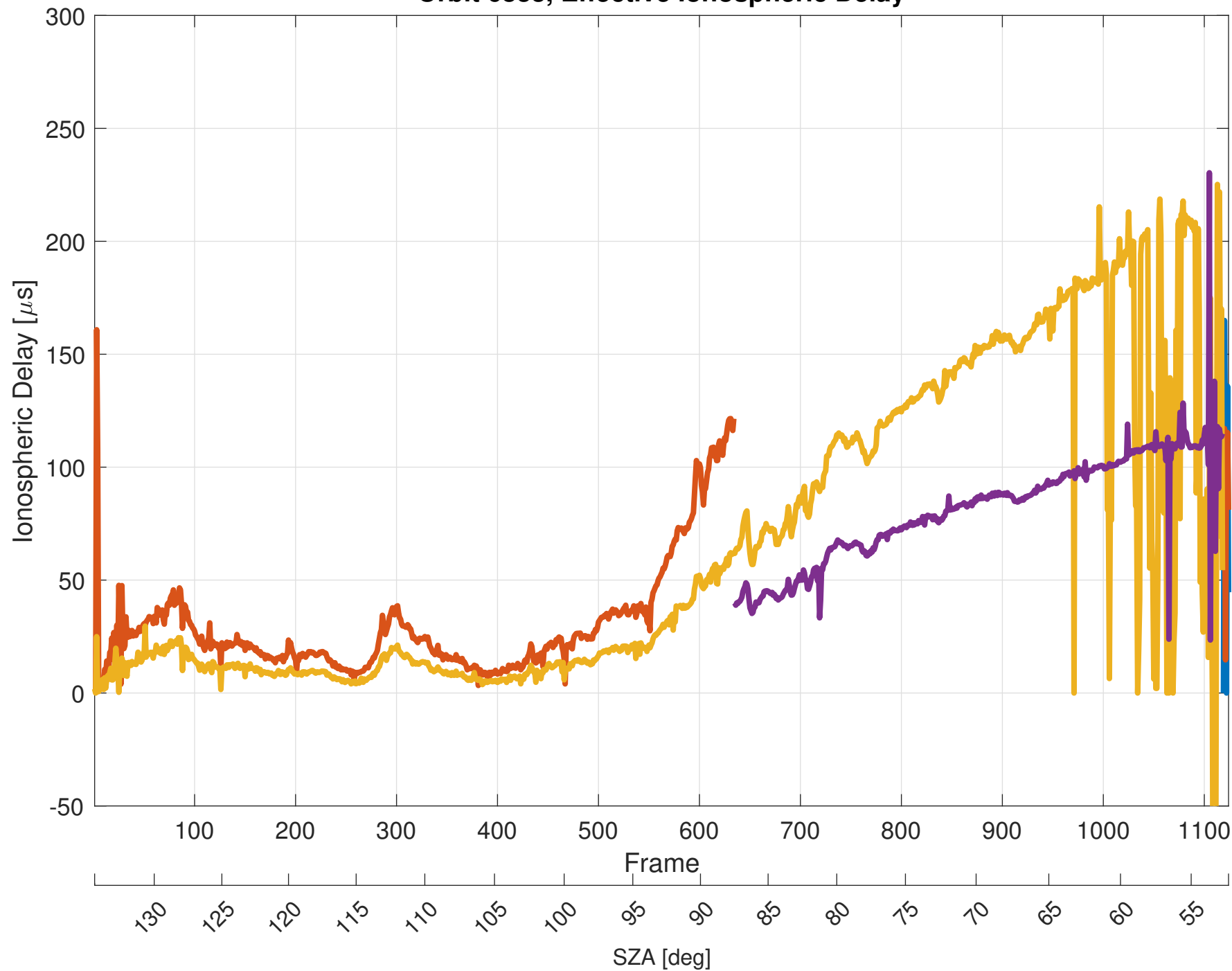
Orbit 6833, Effective Ionospheric Delay
