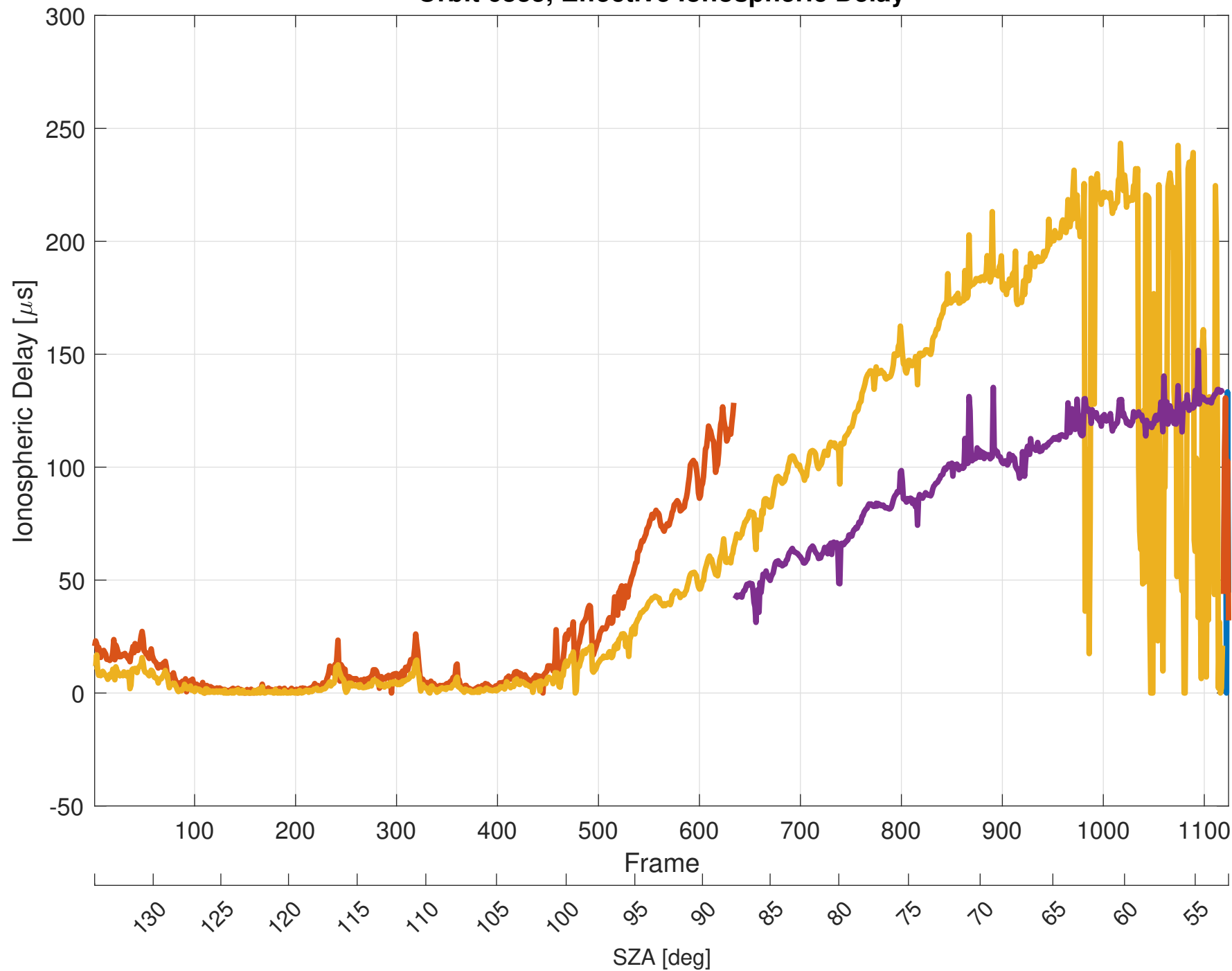
Orbit 6835, Effective Ionospheric Delay
