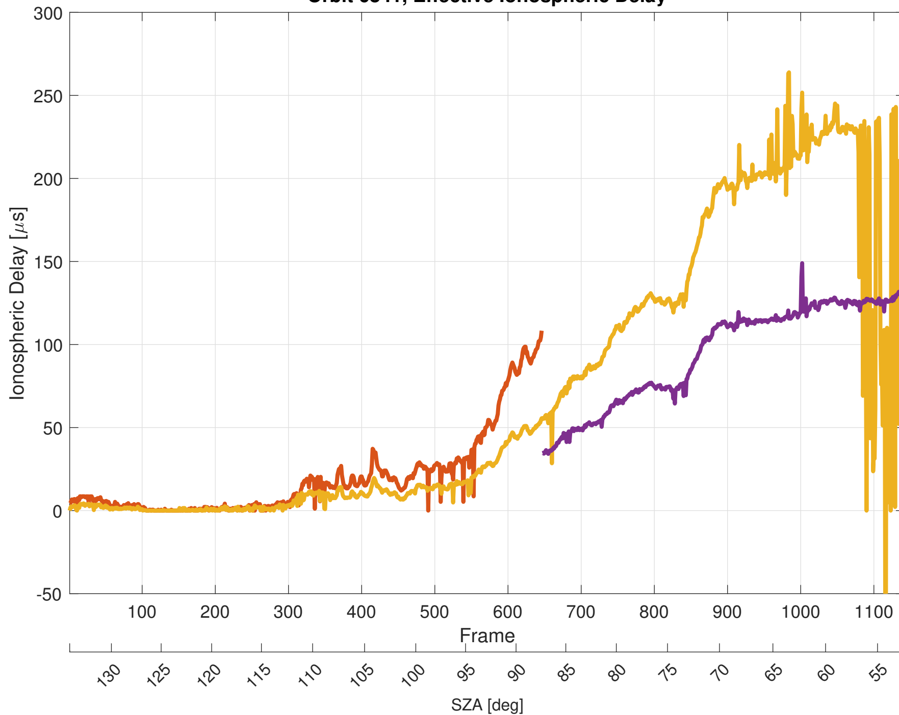
Orbit 6841, Effective Ionospheric Delay
