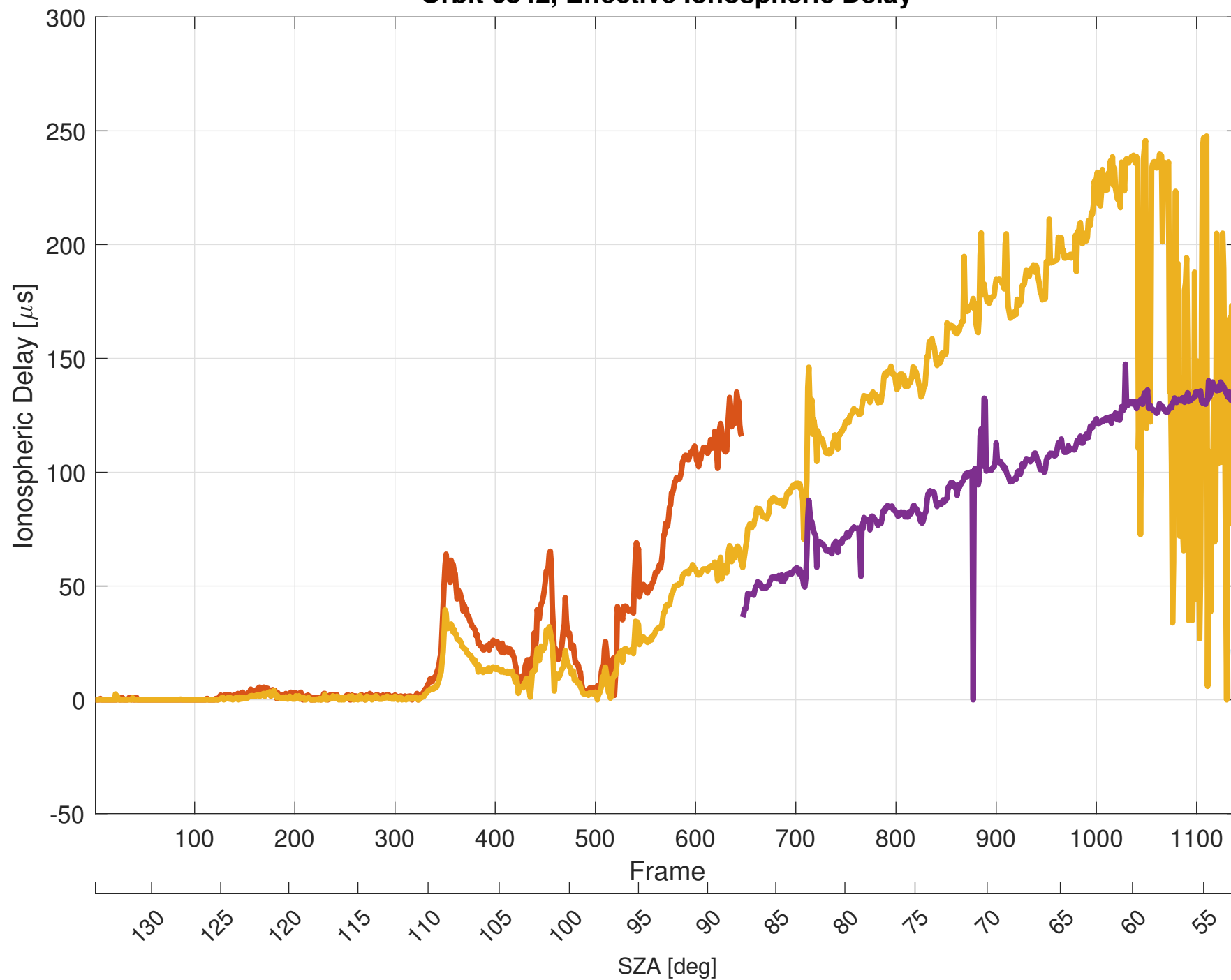
Orbit 6842, Effective Ionospheric Delay
