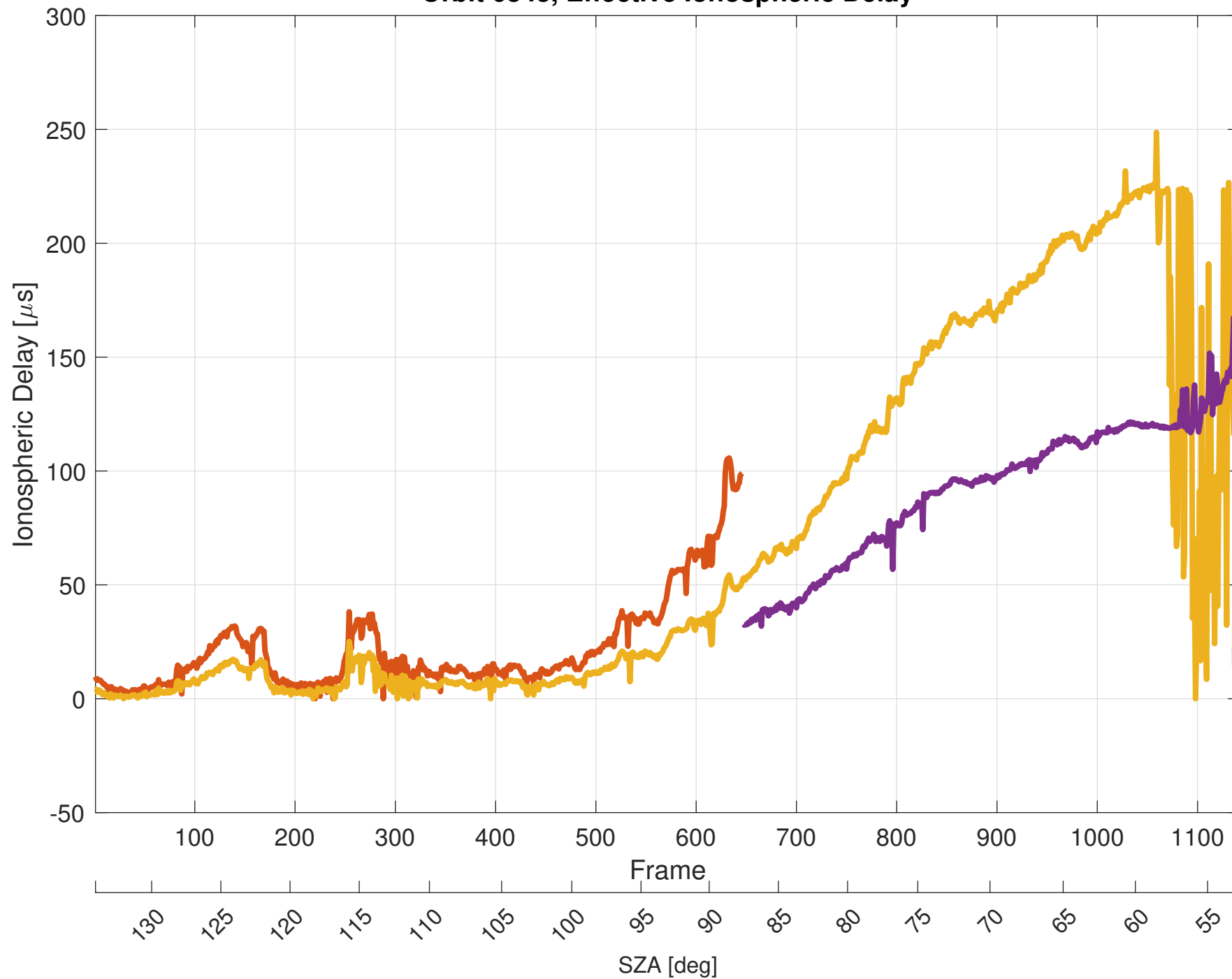
Orbit 6843, Effective Ionospheric Delay
