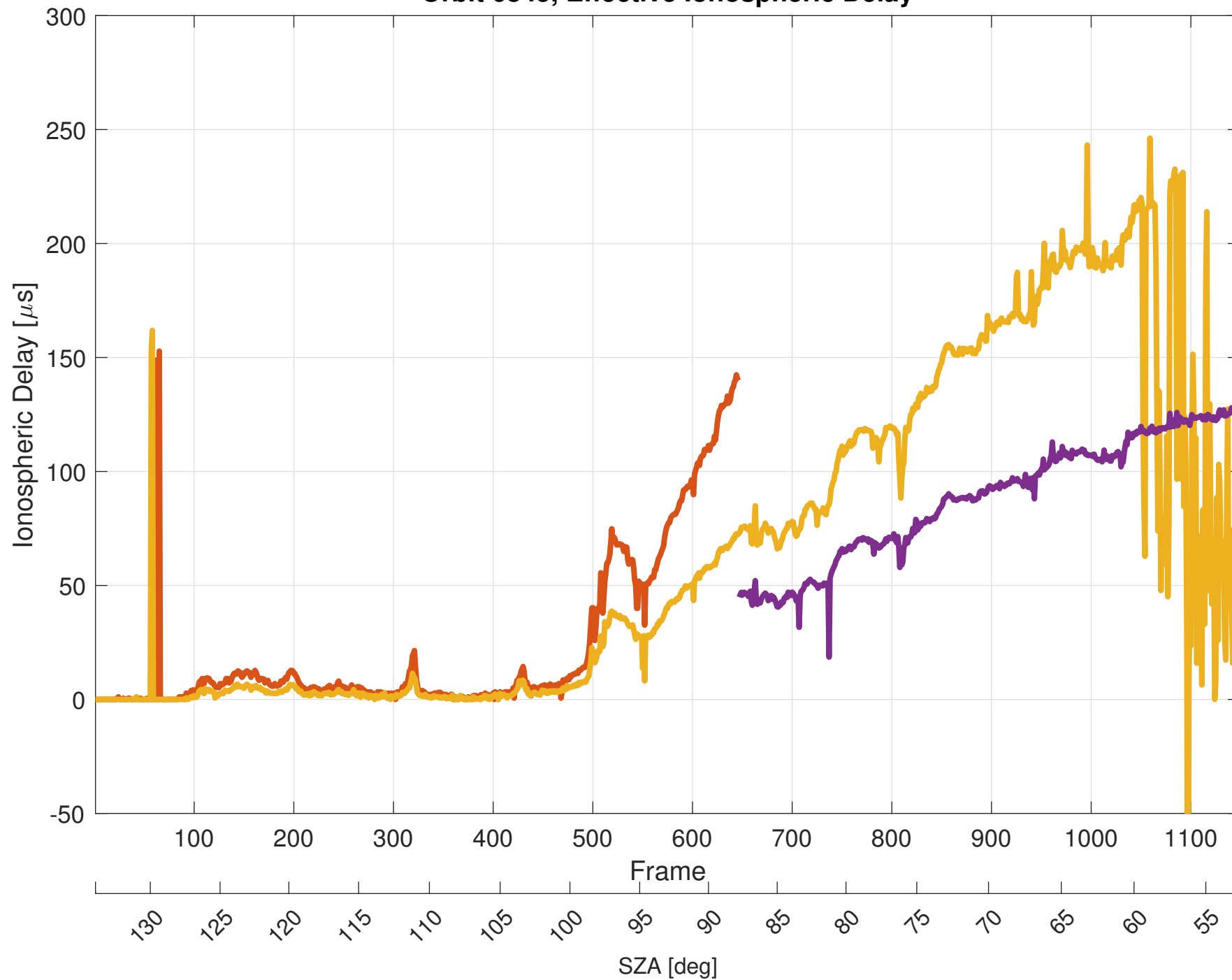
Orbit 6845, Effective Ionospheric Delay
