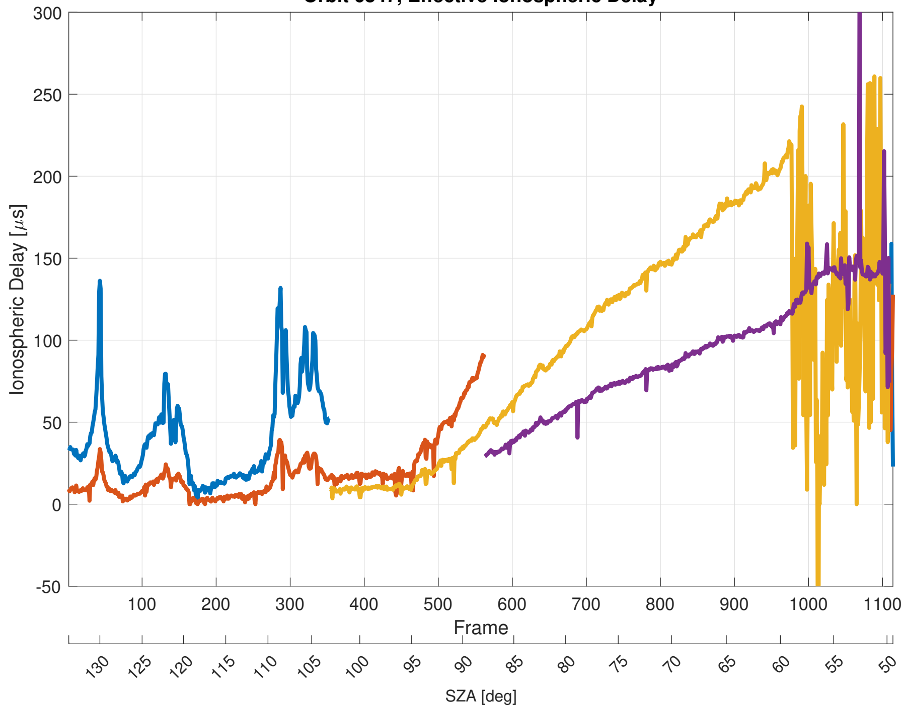
Orbit 6847, Effective Ionospheric Delay
