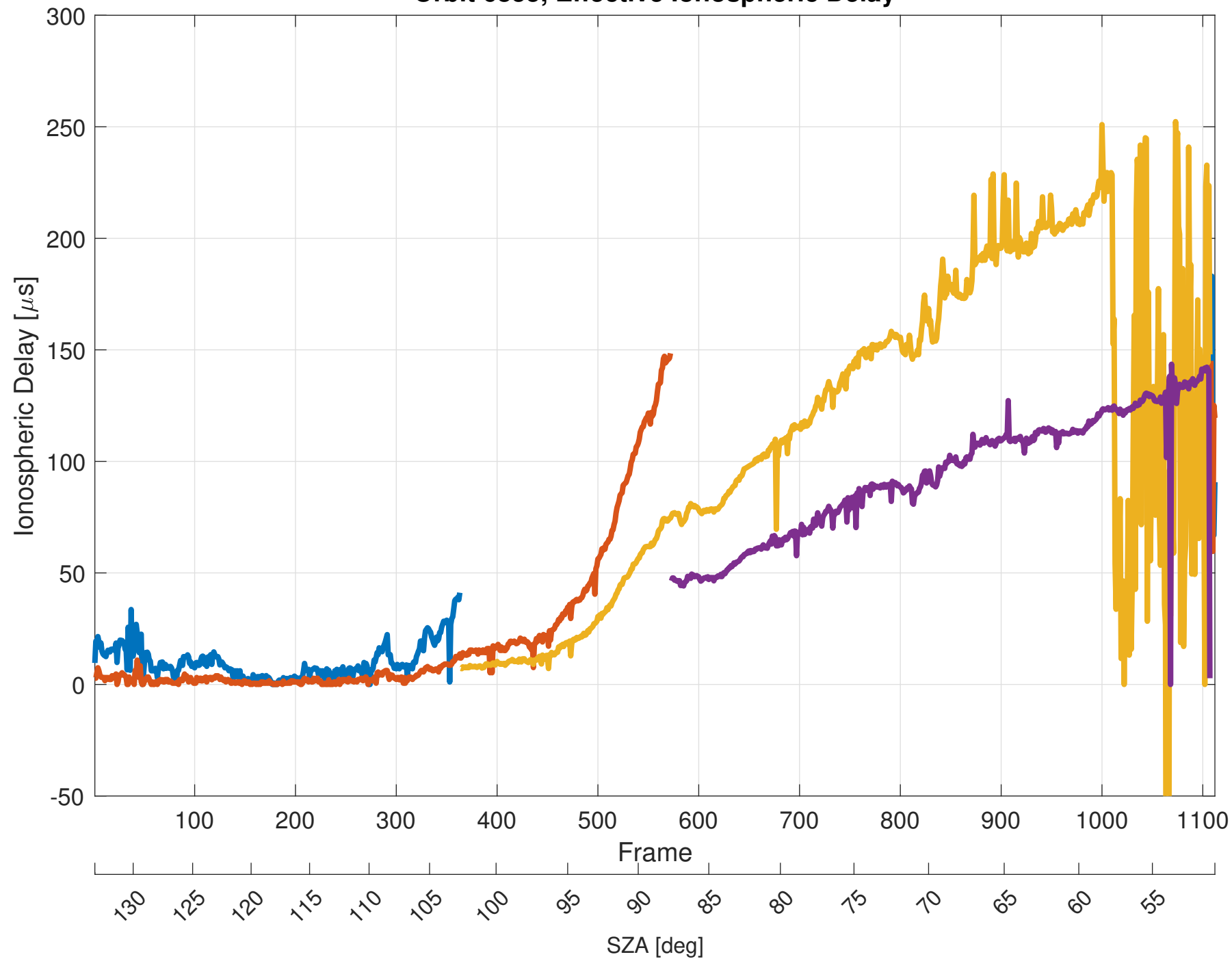
Orbit 6855, Effective Ionospheric Delay
